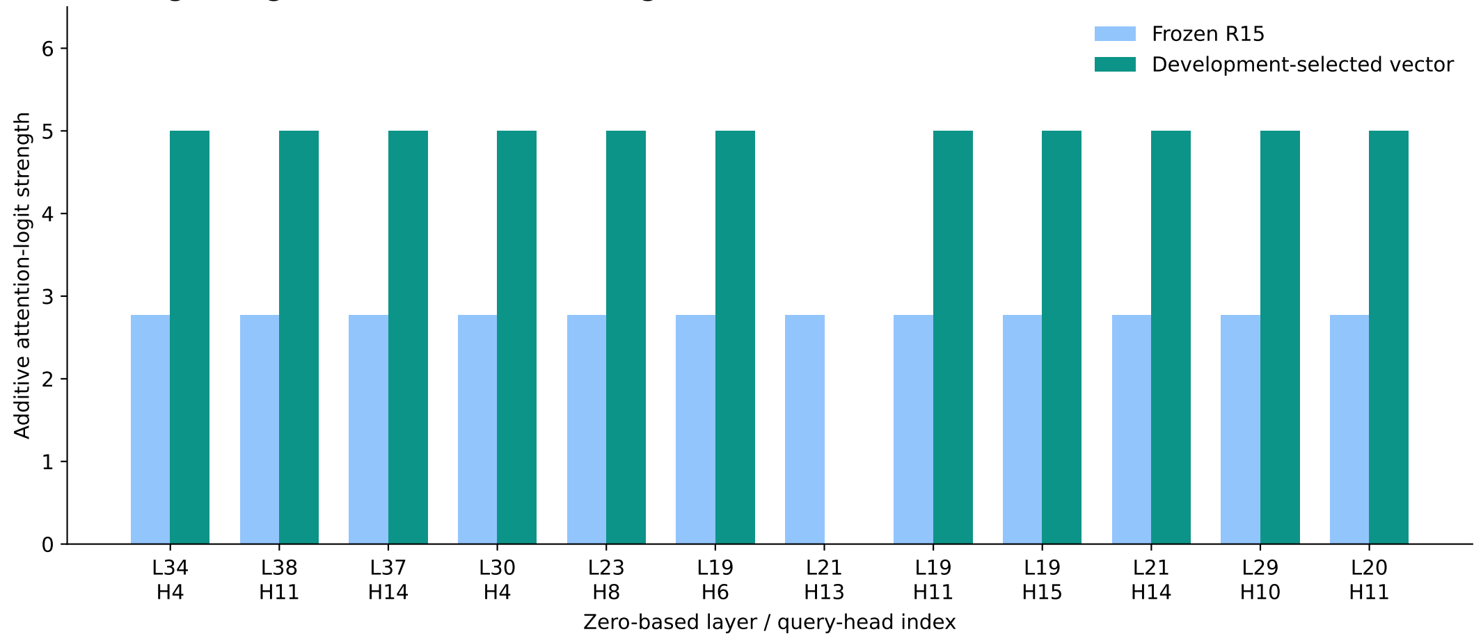
Steering strengths selected before testing
