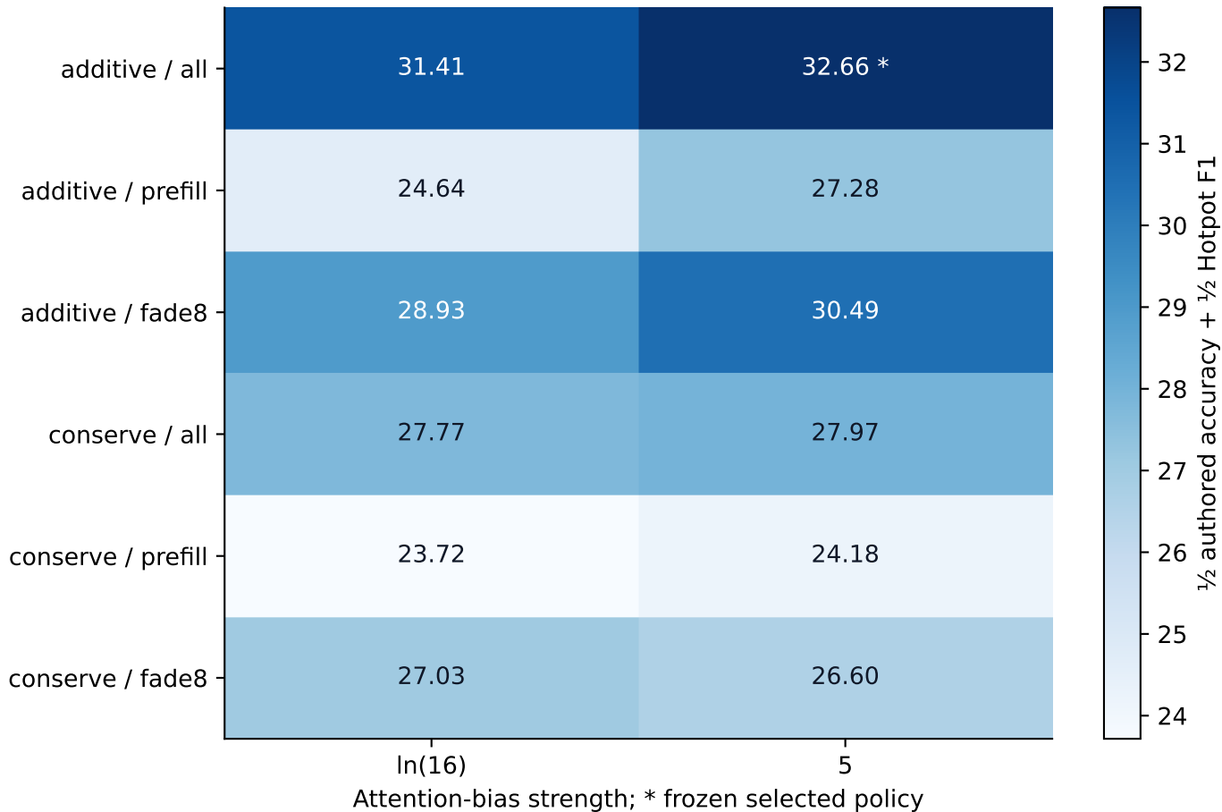
Development search: equal-domain quality (%)
