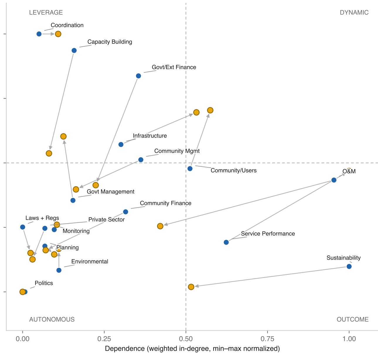
Solution system (min-max scaled, Walters 2022)
