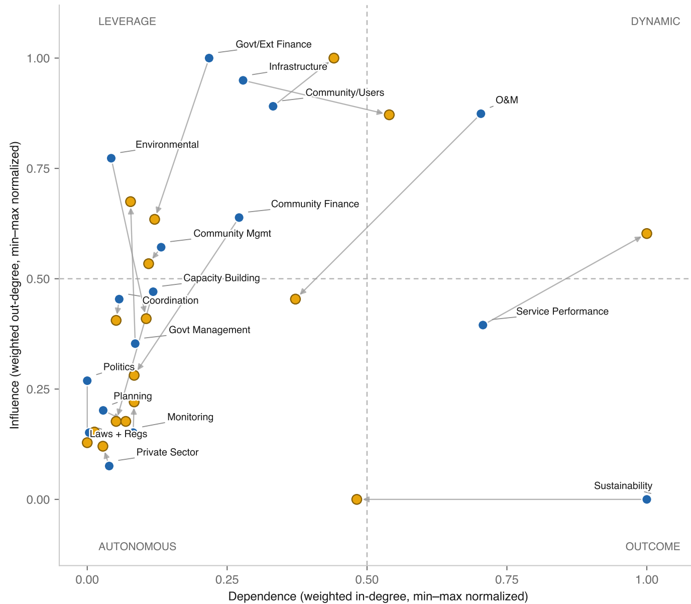
Challenge system (min-max scaled, Walters 2022)
