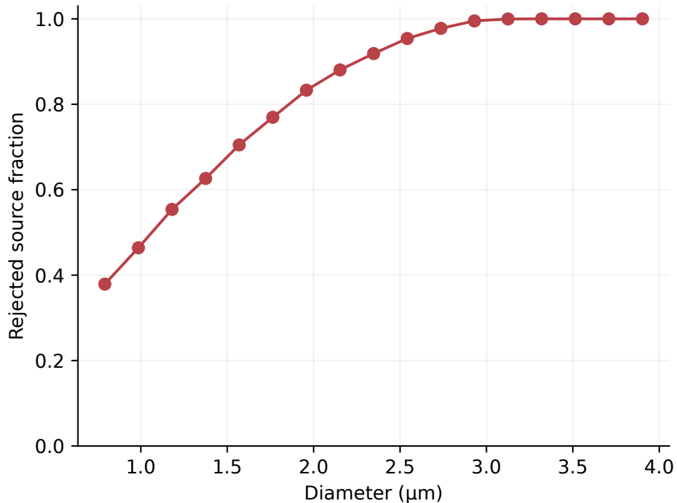
Finite-size rejection vs diameter
