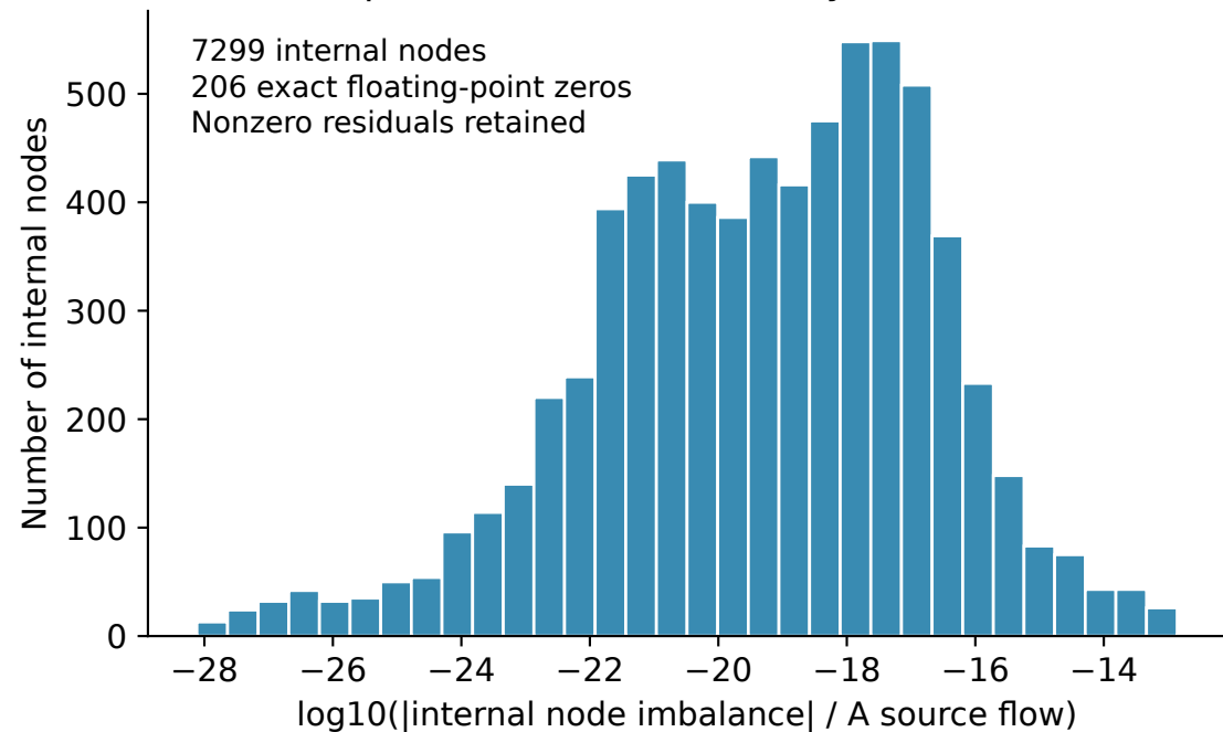
Sparse network continuity residuals
