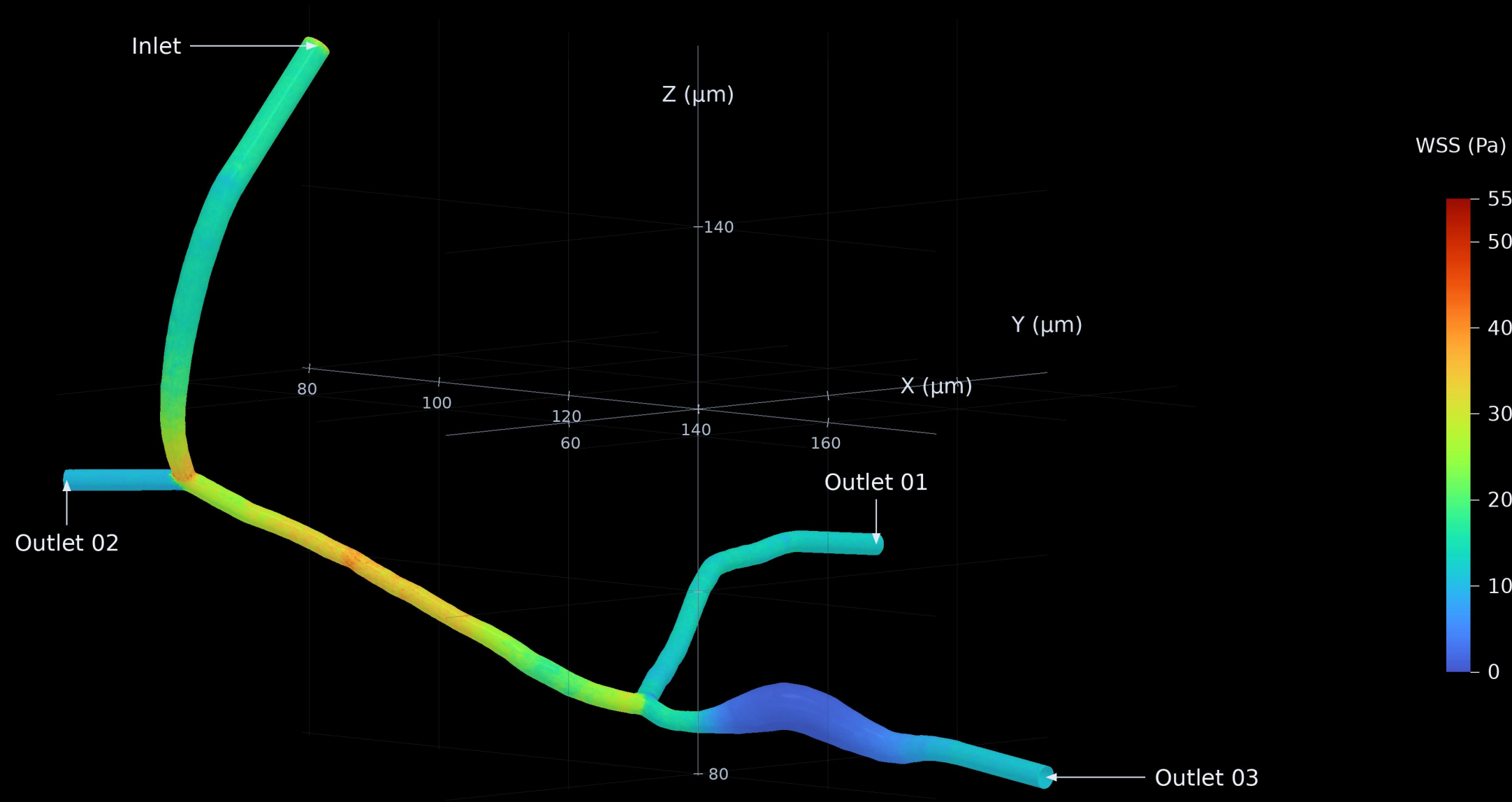
Raw WSS per wall triangle | No nodal averaging
