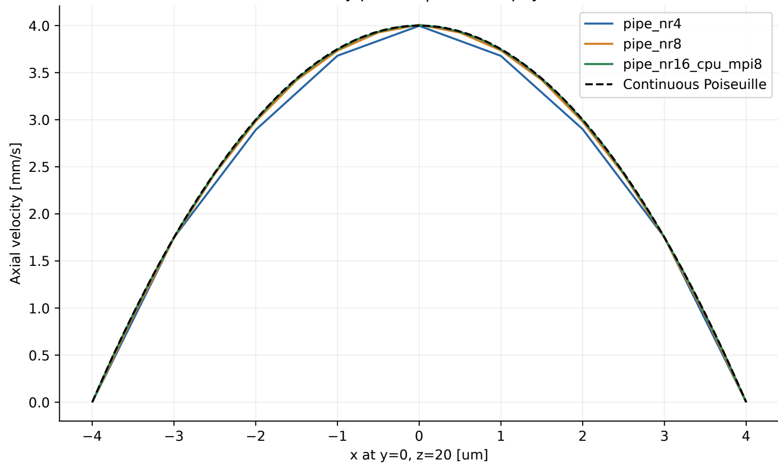
Actual CFD velocity profiles | common physical section
