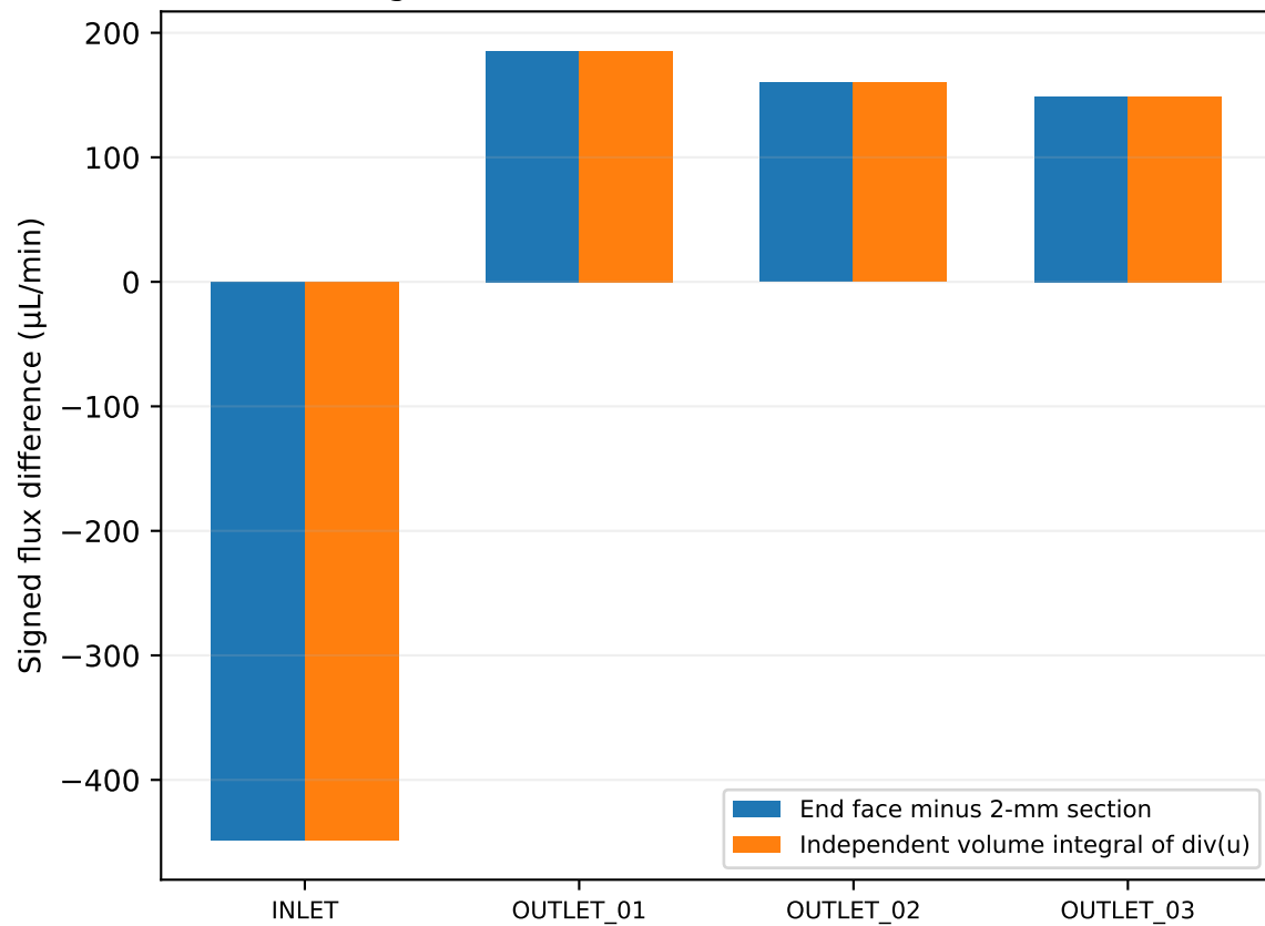
Divergence theorem cross-check of 2-mm slabs
