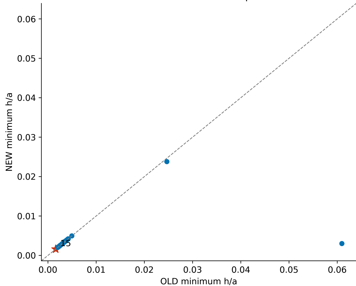
Minimum wall clearance | all 30
