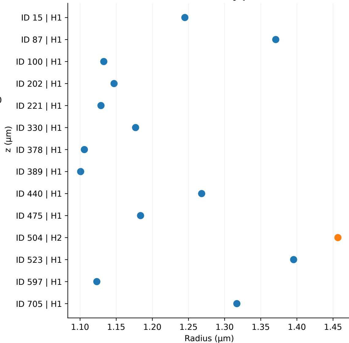
(b) All 14 stationary particles
