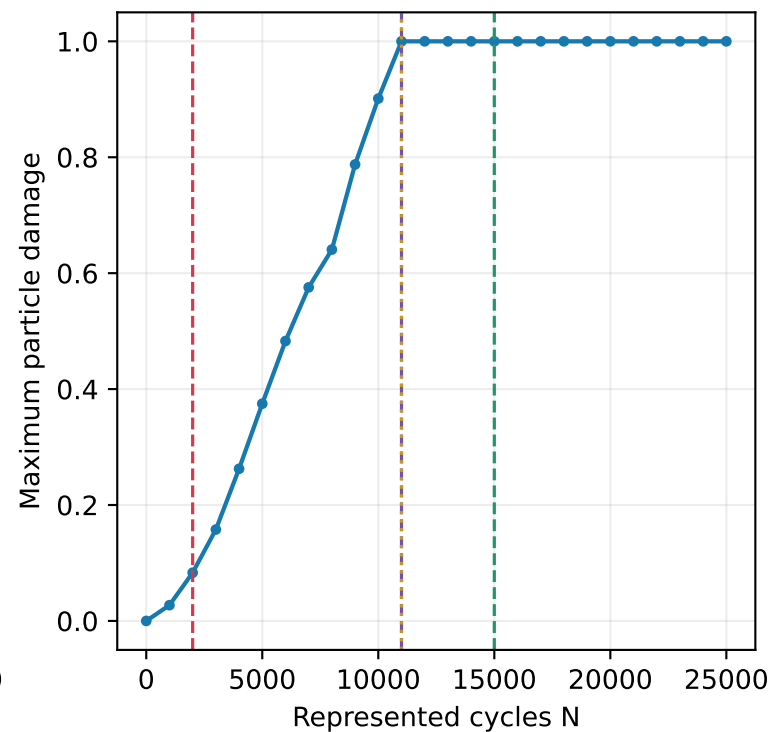
Damage, connectivity and clearance histories
