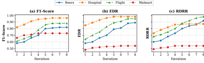
Fig. 5. Performance under different numbers of iterations on datasets Beers, Hospital, Flight, and Walmart. We report F1-Score, EDR, and RDRR in (a)–(c), respectively.
