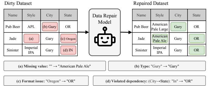
Fig. 1. An illustrated example of common data errors, where (a)–(d) are different types of error. (a) Missing value; (b) Typo; (c) Format Issue; (d) Violated attribute dependency.
