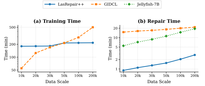
Fig. 9. Scalability of different repair methods under increasing data scales on the Tax dataset.
