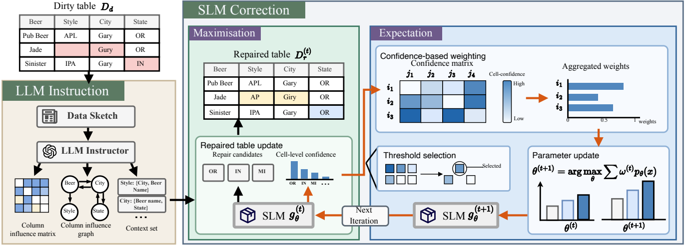
Fig. 3. Overview of LasRepair++. Starting from the dirty table, the LLM instructor constructs a column influence graph and extracts the target-specific context set as repair instructions. The SLM corrector then generates repair candidates and the cell-level confidence. A confidence matrix is then computed and aggregated into confidence-based weights, which are used for updating the parameter. The process terminates when the stop criterion is satisfied and outputs the final repaired table.
