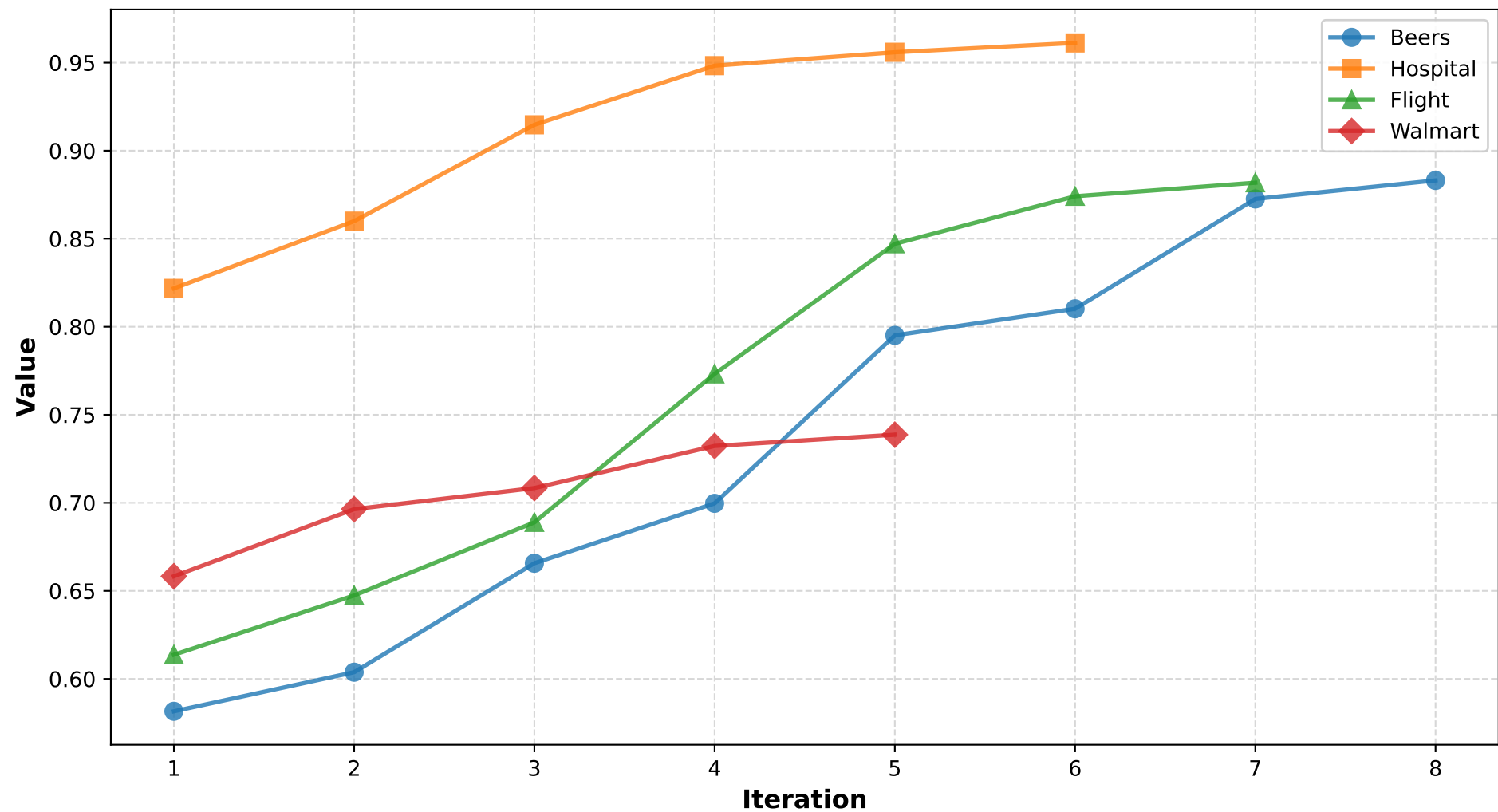
EXP3: Performance Across Different Iterations
