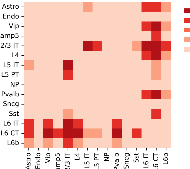
Tangram - BH-Adjusted Pairwise MWU
