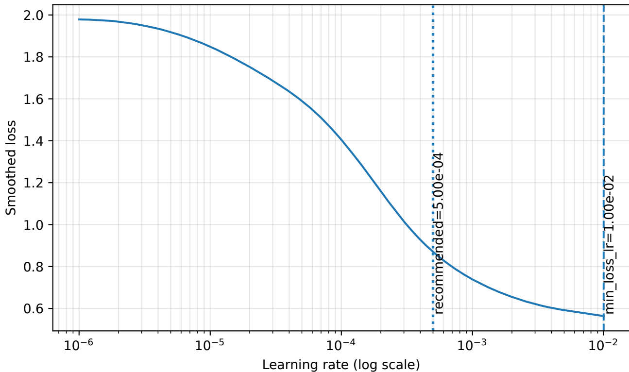
LR Finder (VAE loss)
