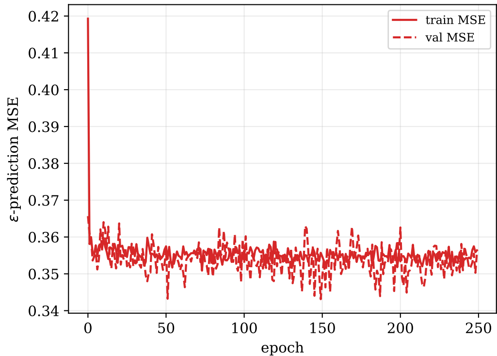
Conditional DDPM training curve
