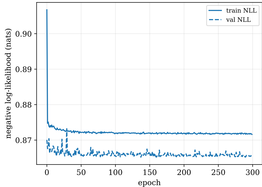
Conditional RealNVP training curve
