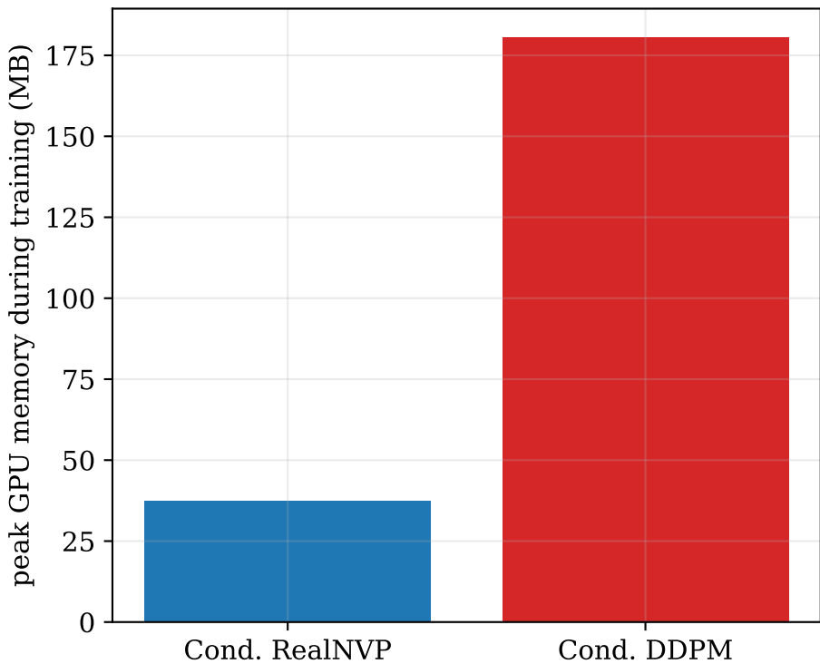
GPU memory usage
