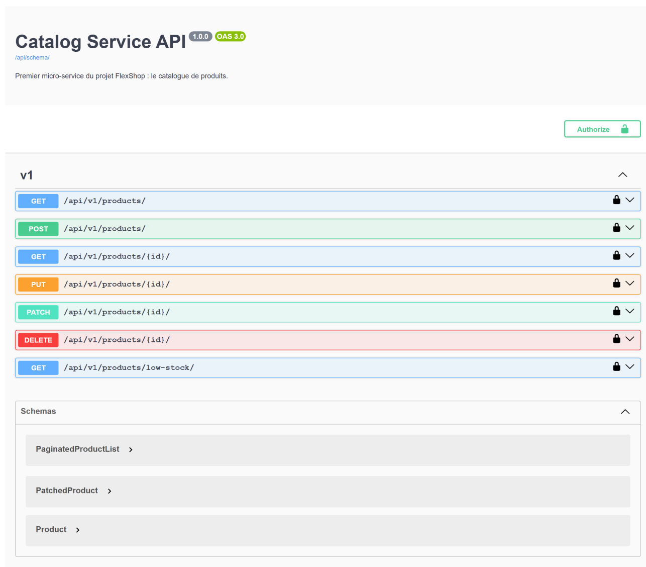
FIGURE 1 – Swagger UI du service Catalogue ( http://localhost:8000/api/docs/ ).
