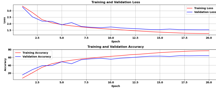
(c) Loss/Accuracy
