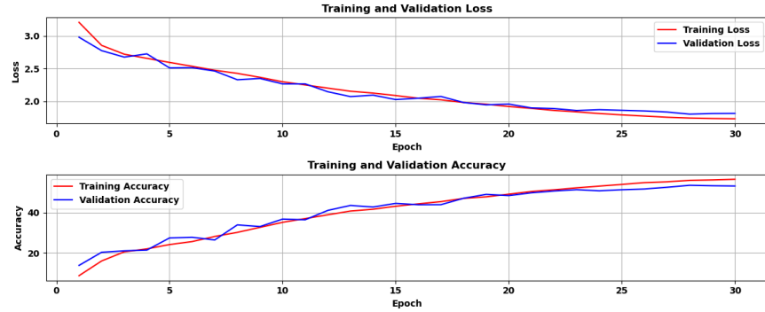
(c) Loss/Accuracy
