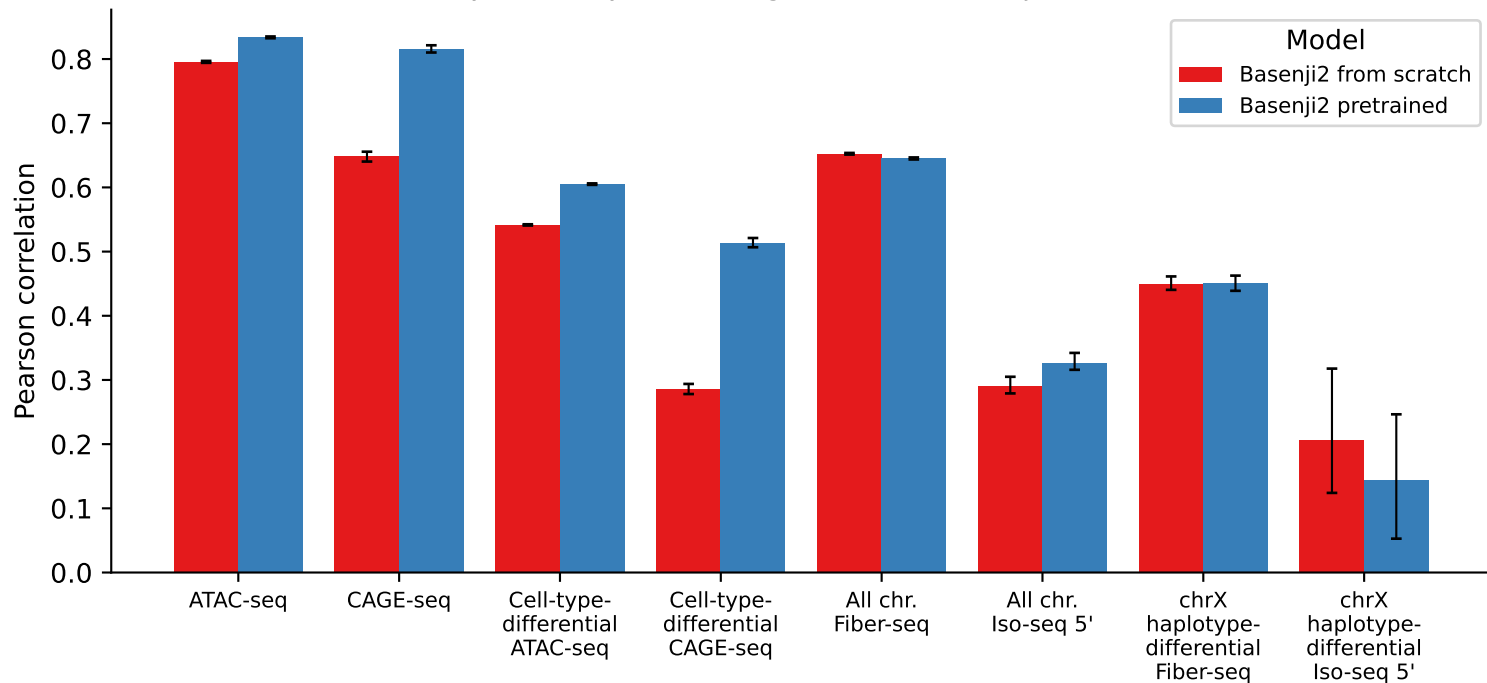
Impacts of pretraining for 22M Basenji2 model
