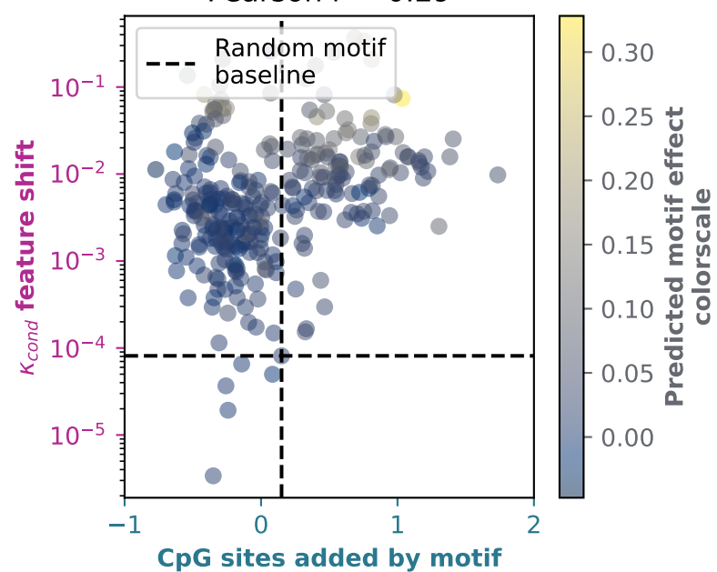
CpGs added vs reps shift Pearson r = 0.29
