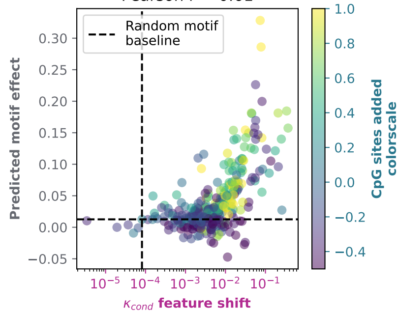
Rep shift vs preds effect Pearson r = 0.61
