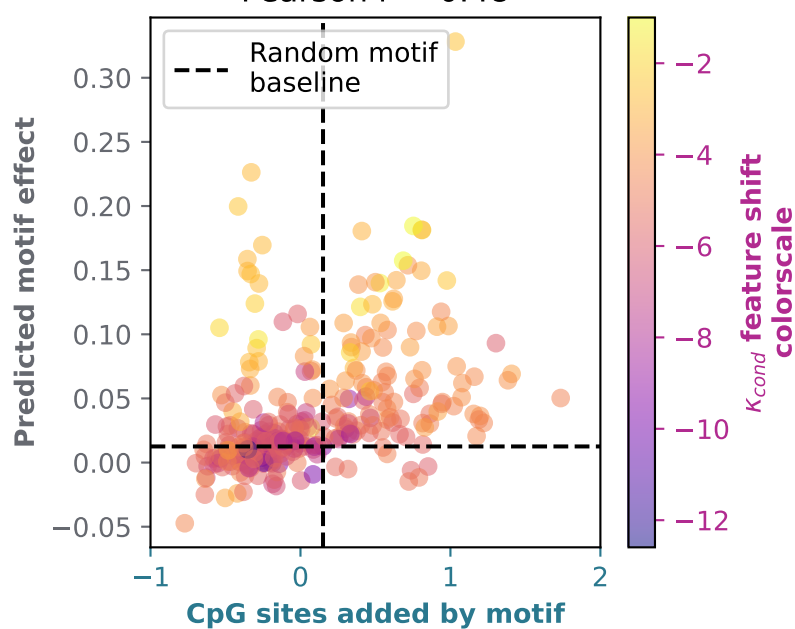
CpGs added vs preds effect Pearson r = 0.48
