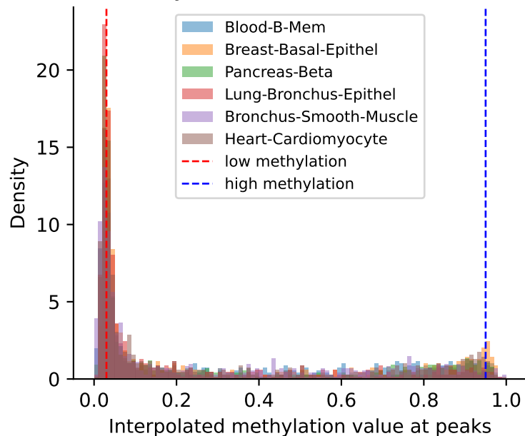
Methylation fraction distribution
