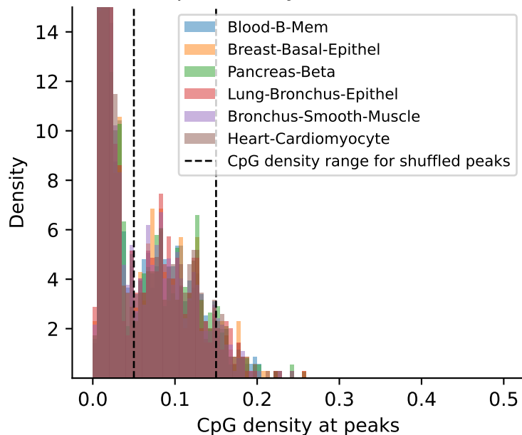
CpG density distribution
