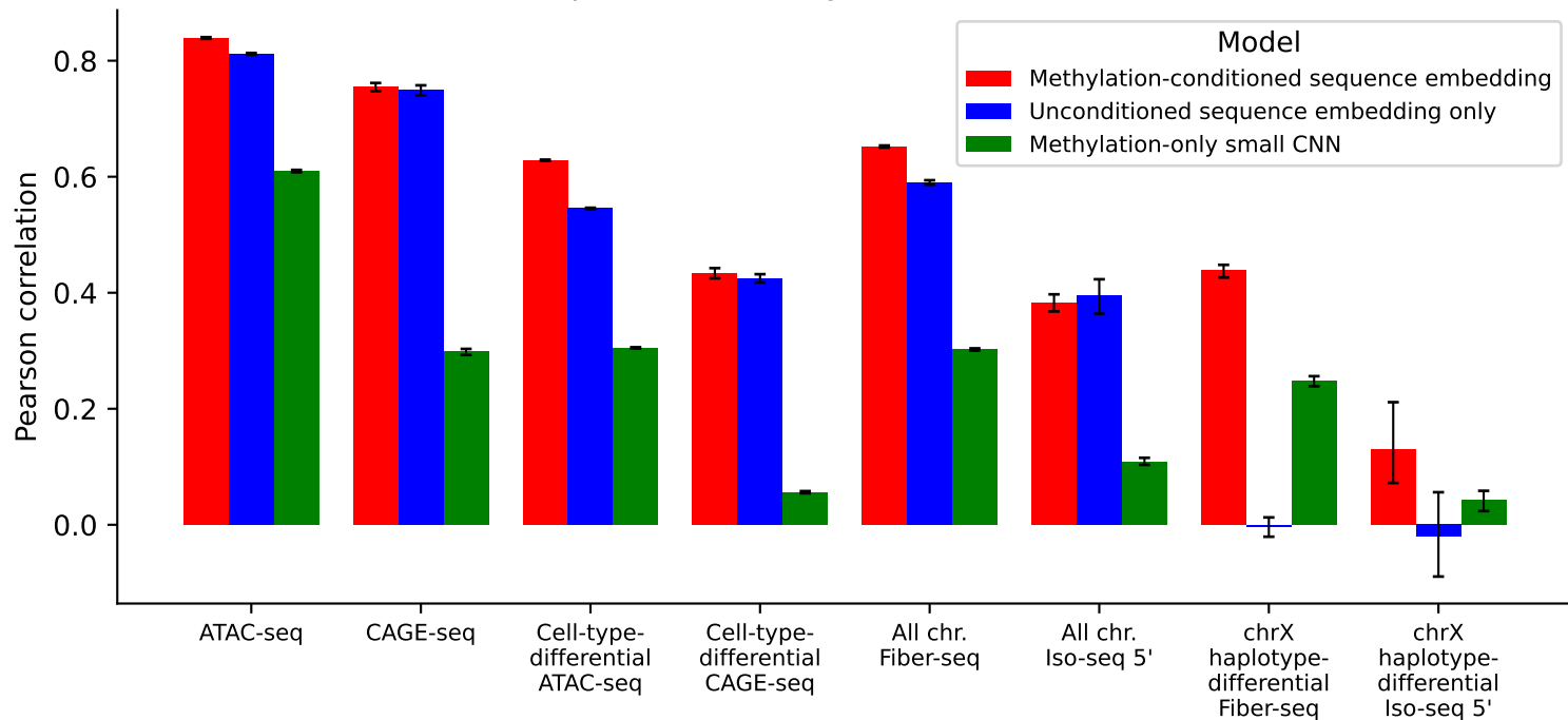
Sequence vs Methylation contributions
