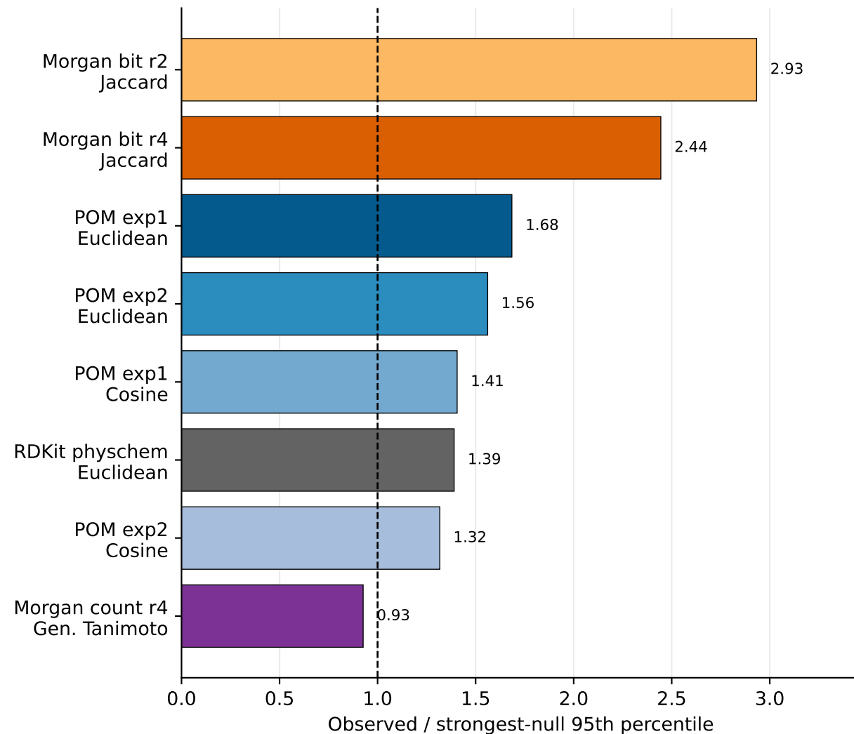
Curated 4,983-row GS/LF table Direct repeated-subsample H1
