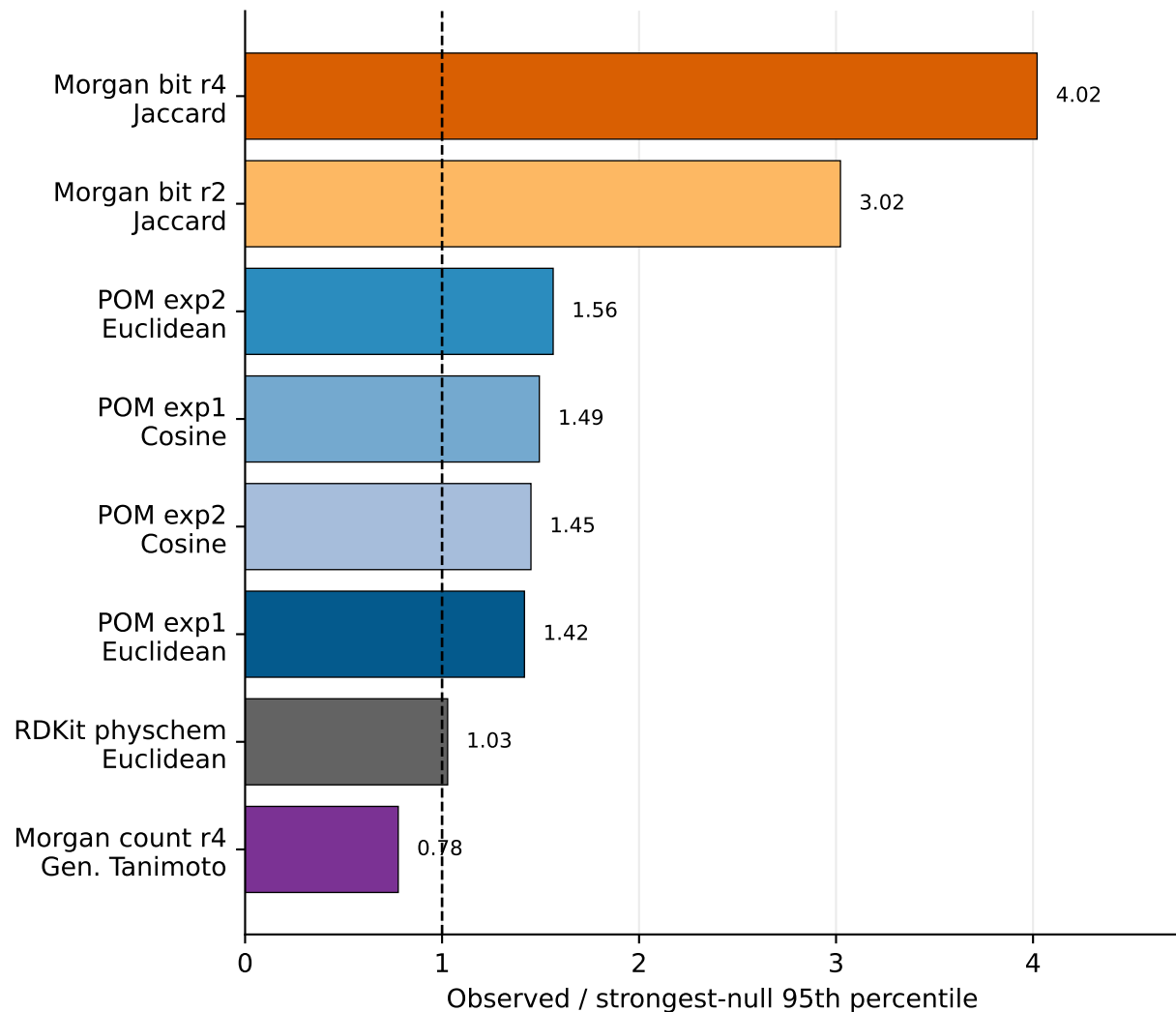
1,600-molecule non-overlap subset Direct repeated-subsample H1
