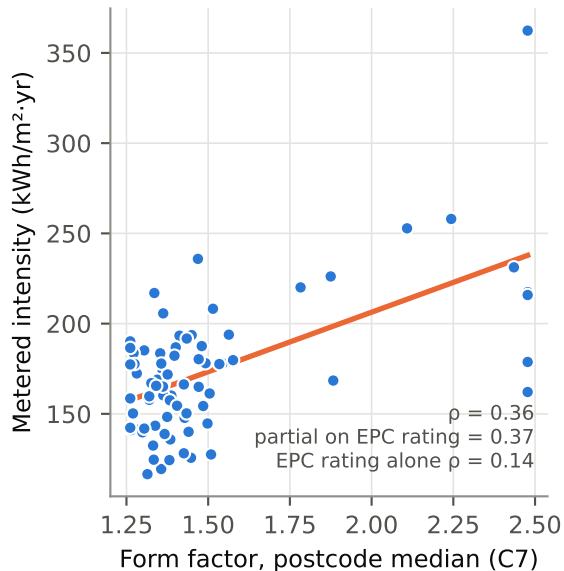
b Form factor vs metered intensity
