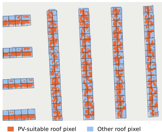
b Roof slope and aspect → PV area (C8)
