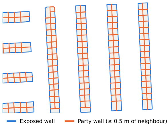
c Exposed and party walls → form factor (C7)
