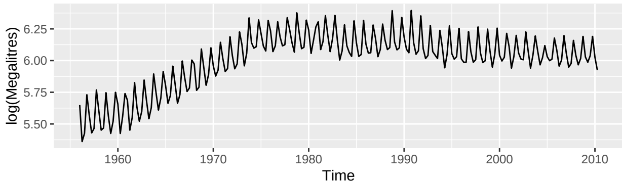
Log-transformed series
