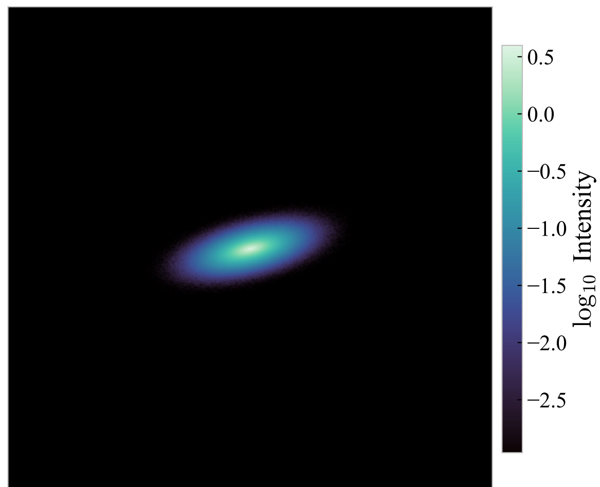
Disc Model
