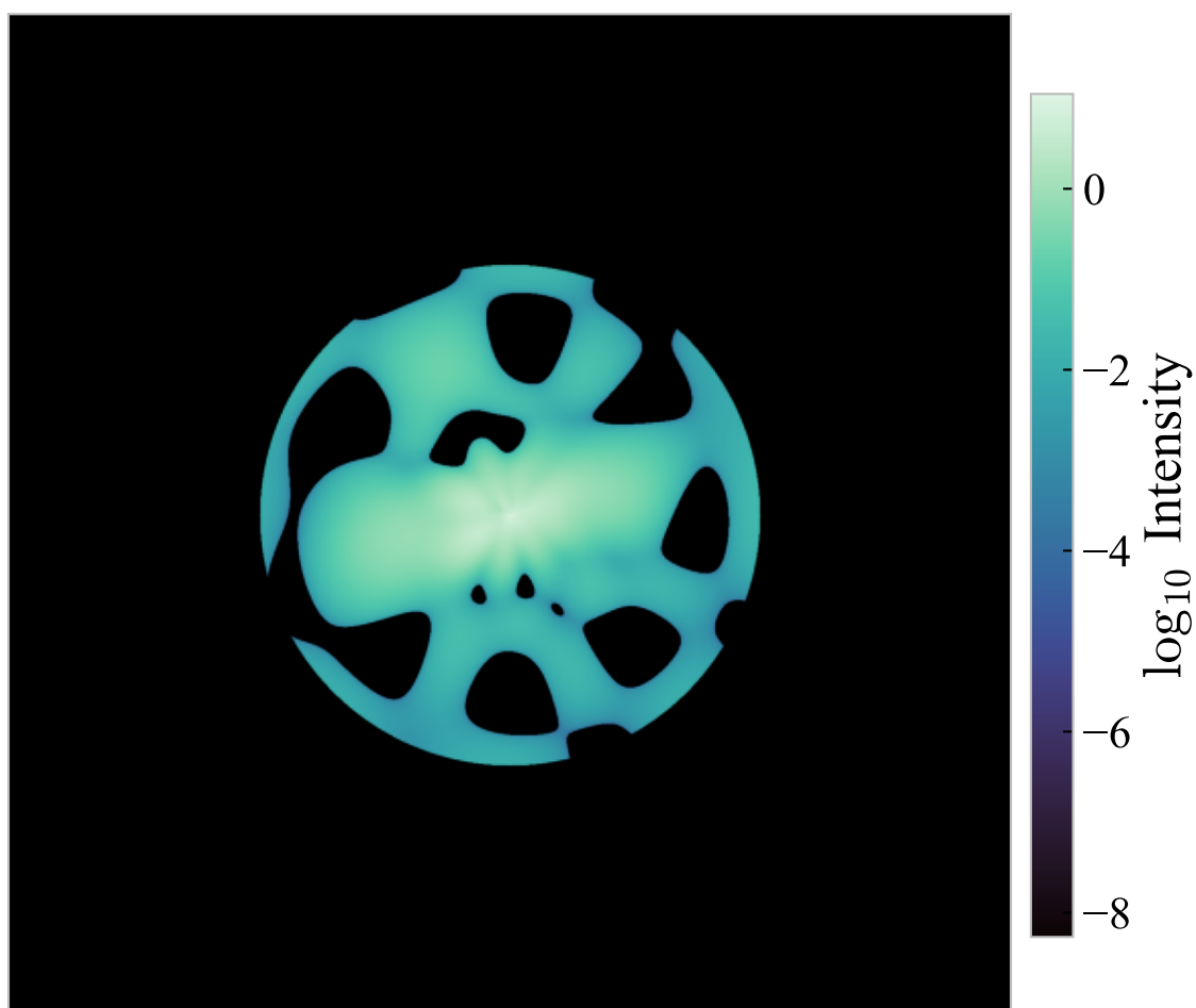
FLEX Reconstruction
