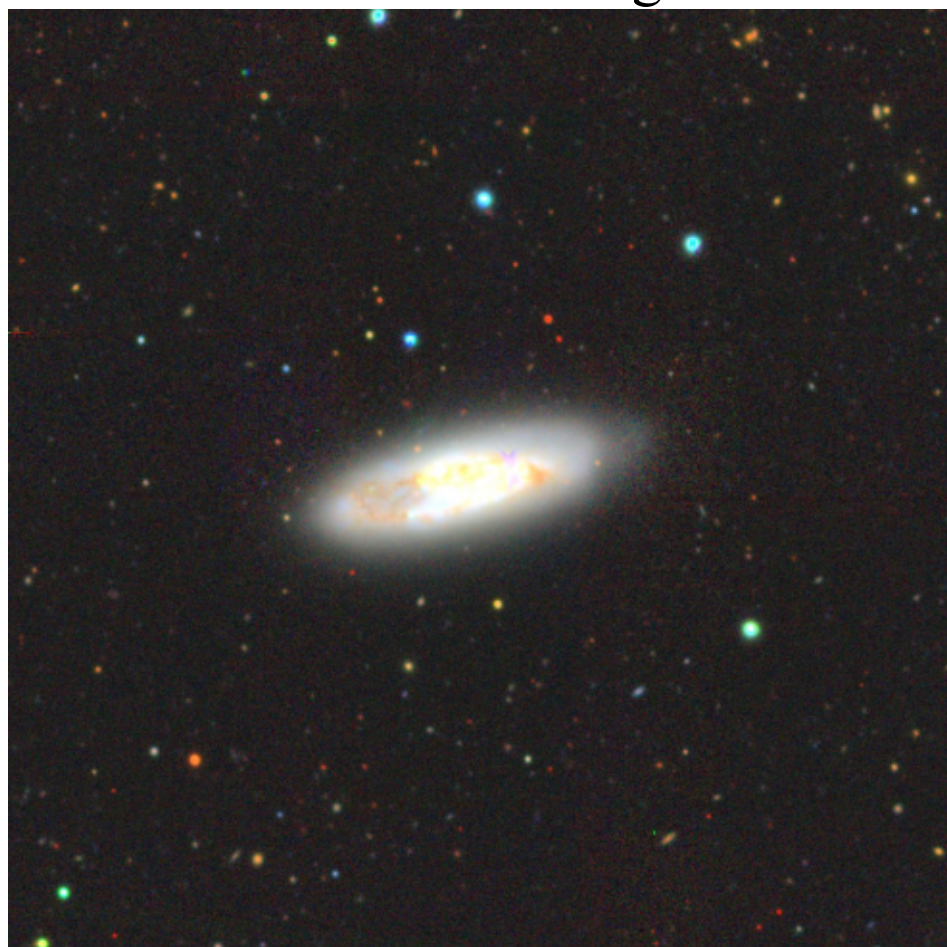
NGC3067 Image
