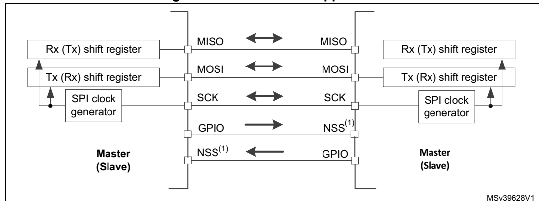
Figure 577. Multi-master application
