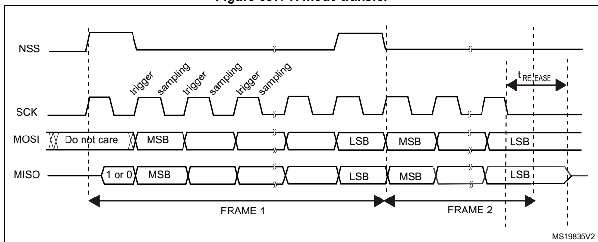
Figure 587. TI mode transfer
