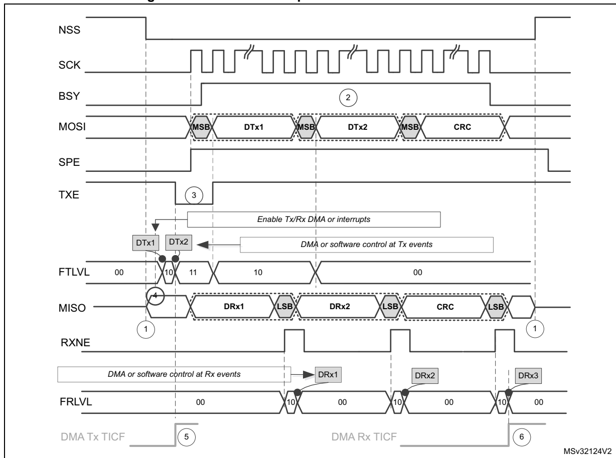
Figure 584. Master full-duplex communication with CRC
