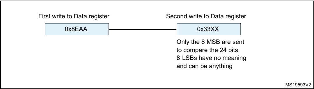
Figure 591. Transmitting 0x8EAA33
