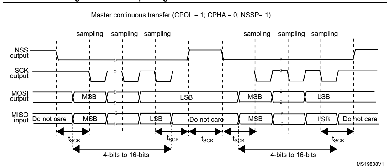
Figure 586. NSSP pulse generation in Motorola SPI master mode
