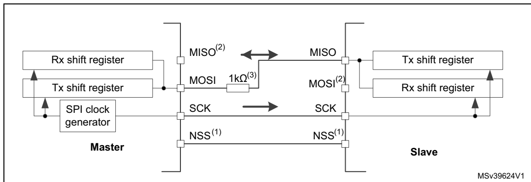
Figure 574. Half-duplex single master/ single slave application
