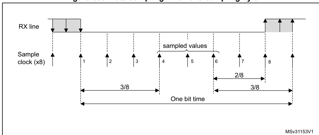
Figure 538. Data sampling when oversampling by 8
