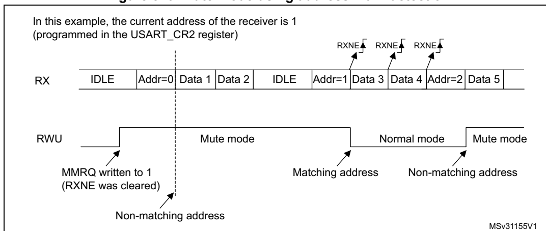
Figure 540. Mute mode using address mark detection
