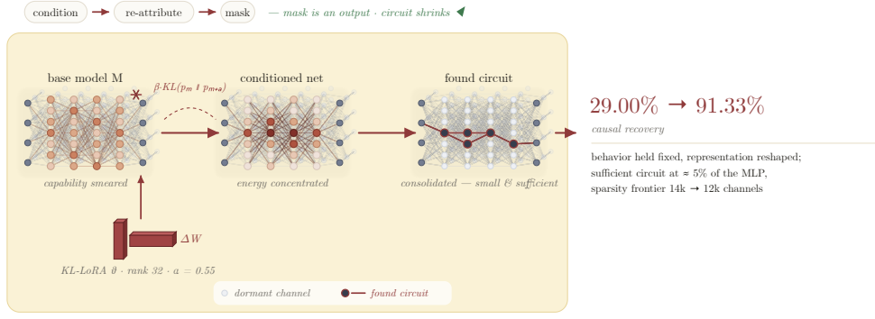
Figure 5: Low-rank collimation (pre-attribution) . A rank-32, KL-constrained LoRA adapter trains on the full, unmasked model under \mathcal{L} = \mathcal{L}_{\text{task}} + \beta \text{KL}(p_M \| p_{M_\theta}) , then merges at the lowest-KL scale ( \alpha=0.55 ). Behavior is held fixed while the representation is reshaped, concentrating task-relevant energy into a compact set of channels. Attribution is run afterward : the mask is an output of collimation. The sparsity frontier moves left—the sufficient circuit shrinks ( \approx 14\text{k} \rightarrow 12\text{k} channels) and causal recovery rises from 29.00% \rightarrow 91.33% at \approx 5\% of the MLP.
