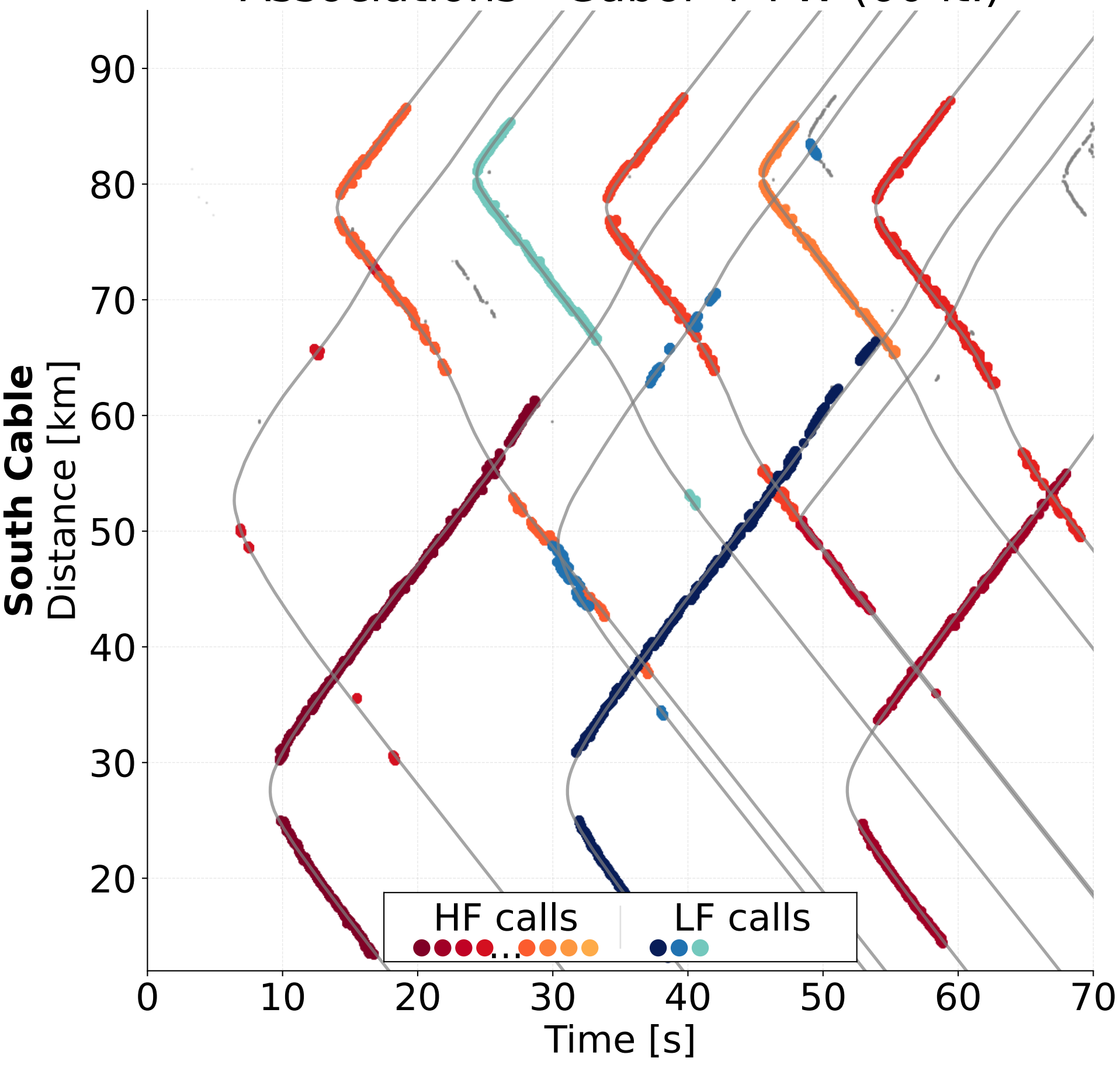
Associations - Gabor + FW (60 it.)
