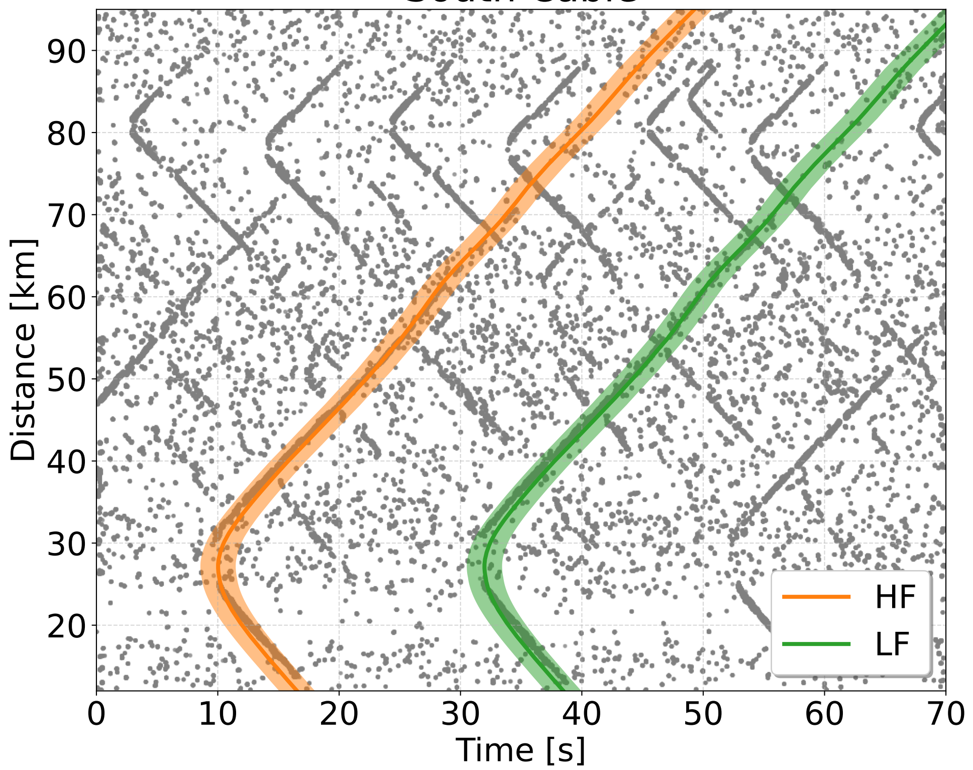
South Cable
