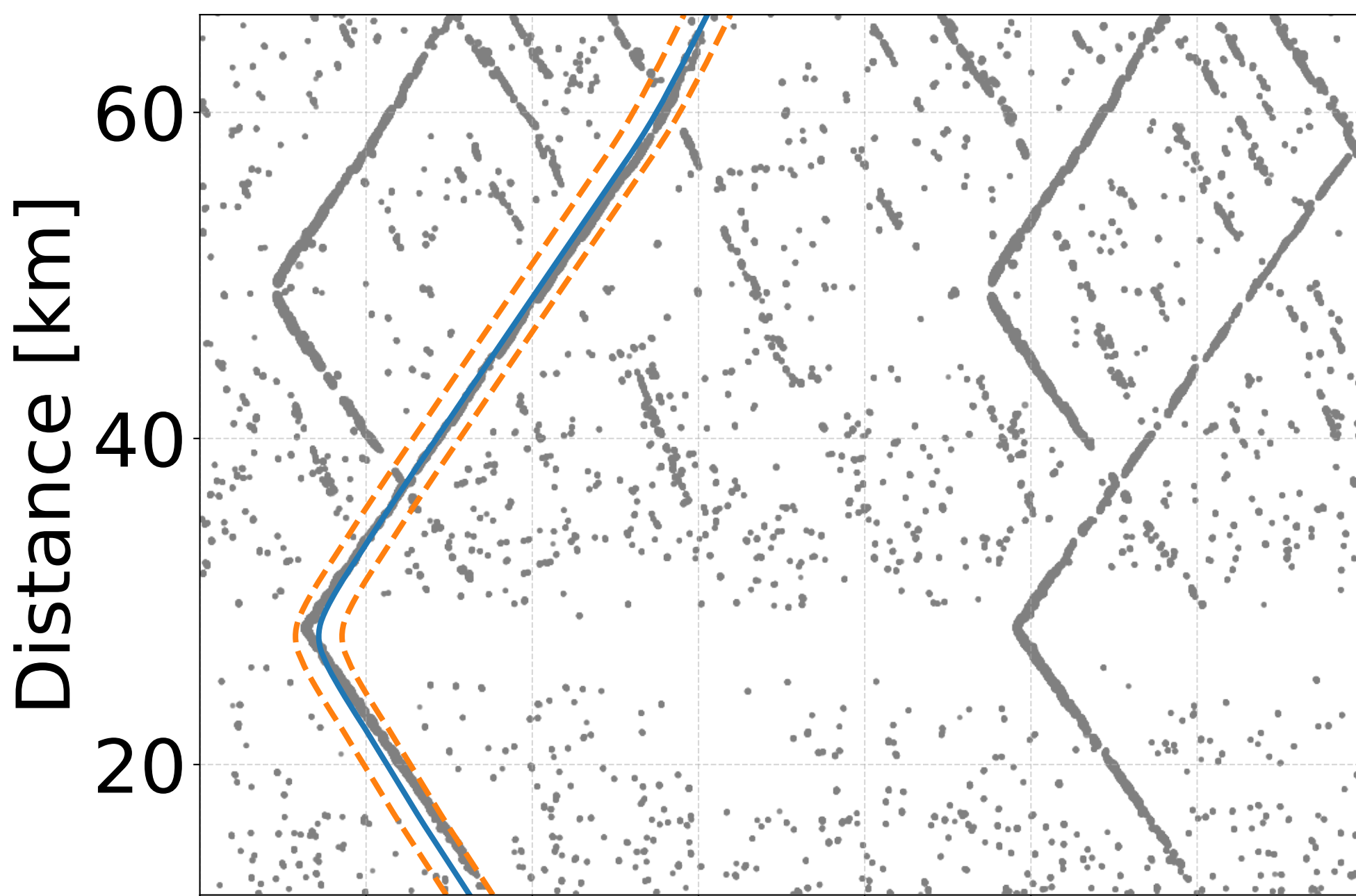
South Cable - HF
