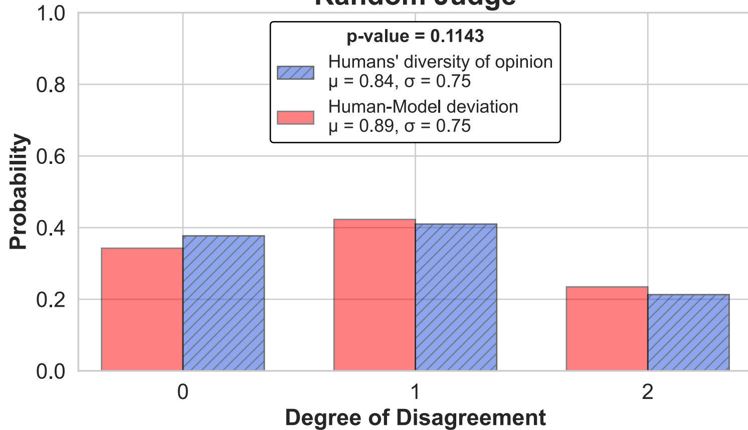
Random Judge
