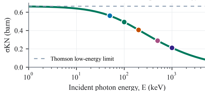
(c) Total cross-section falls with photon energy
