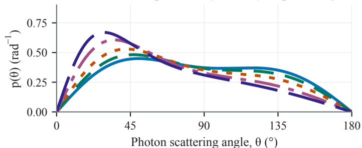
(b) Normalized probability density in polar angle
