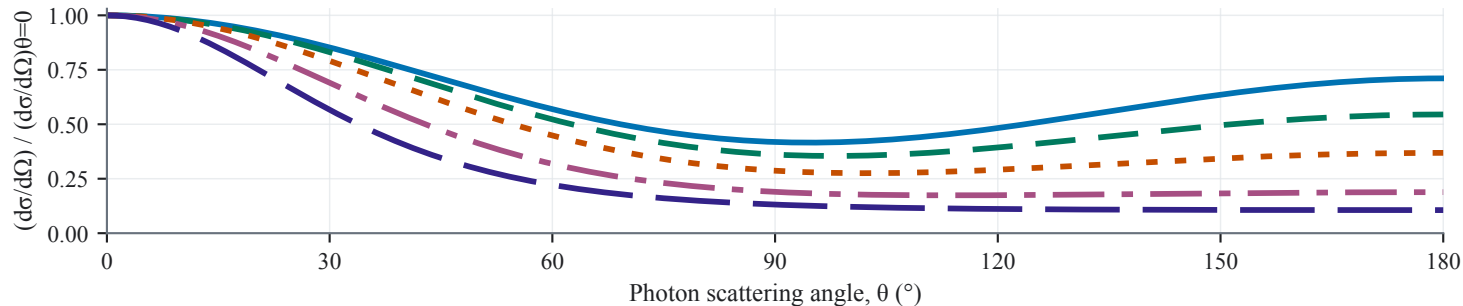
(b) Normalized probability density in polar angle
