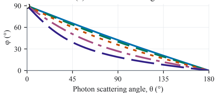
(c) Electron recoil angle
