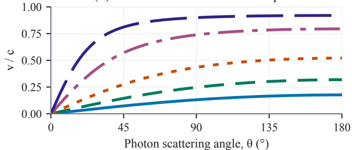
(b) Relativistic electron recoil speed
