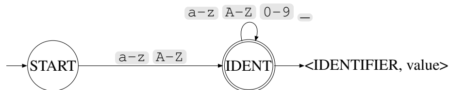
Figure 2.1: DFA for identifiers, keywords, and type names.
