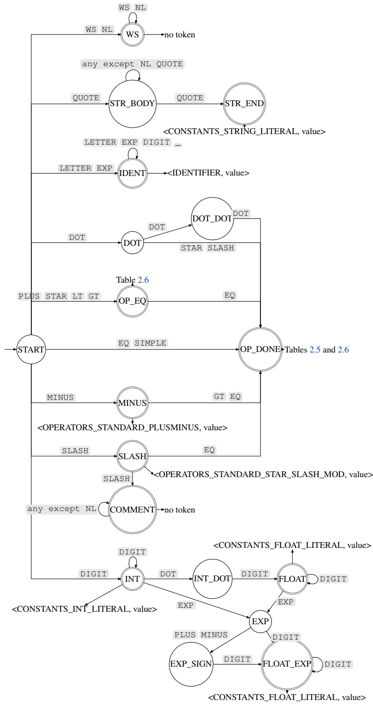
Figure 2.7: The merged DFA of the lexer.
