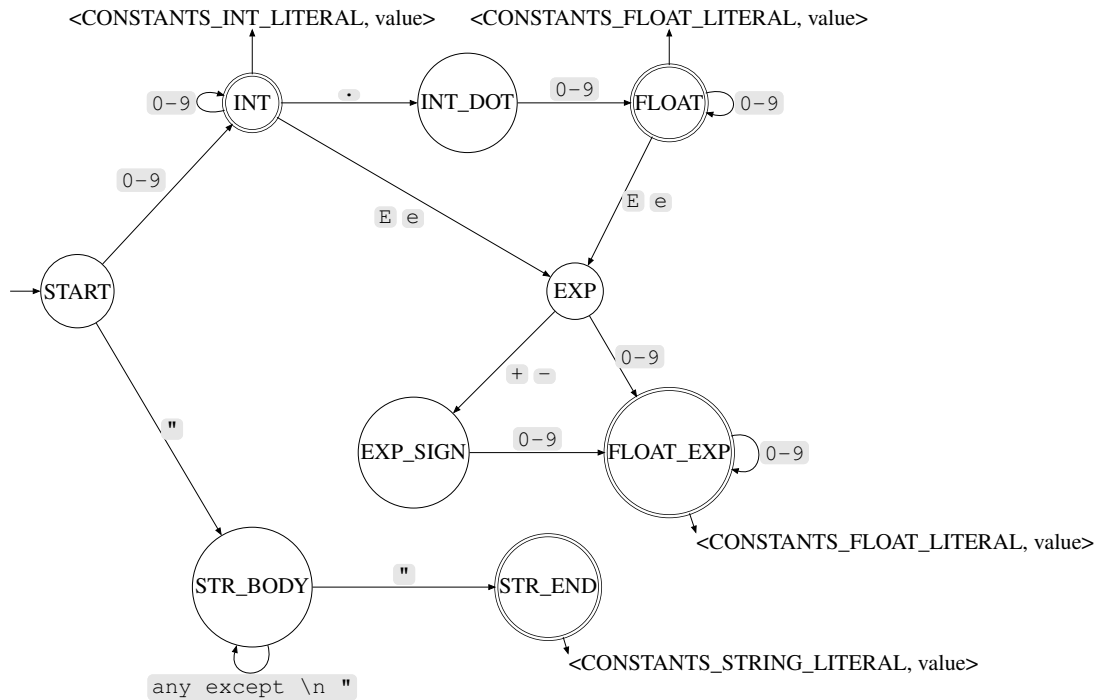
Figure 2.4: DFA for constants.
