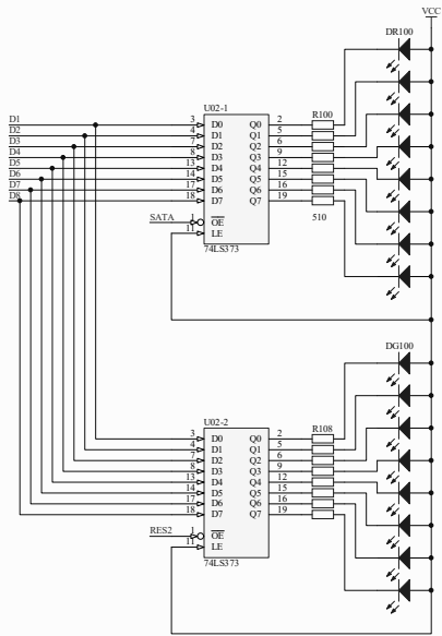
PART-02-抢答者指示电路R100-149
