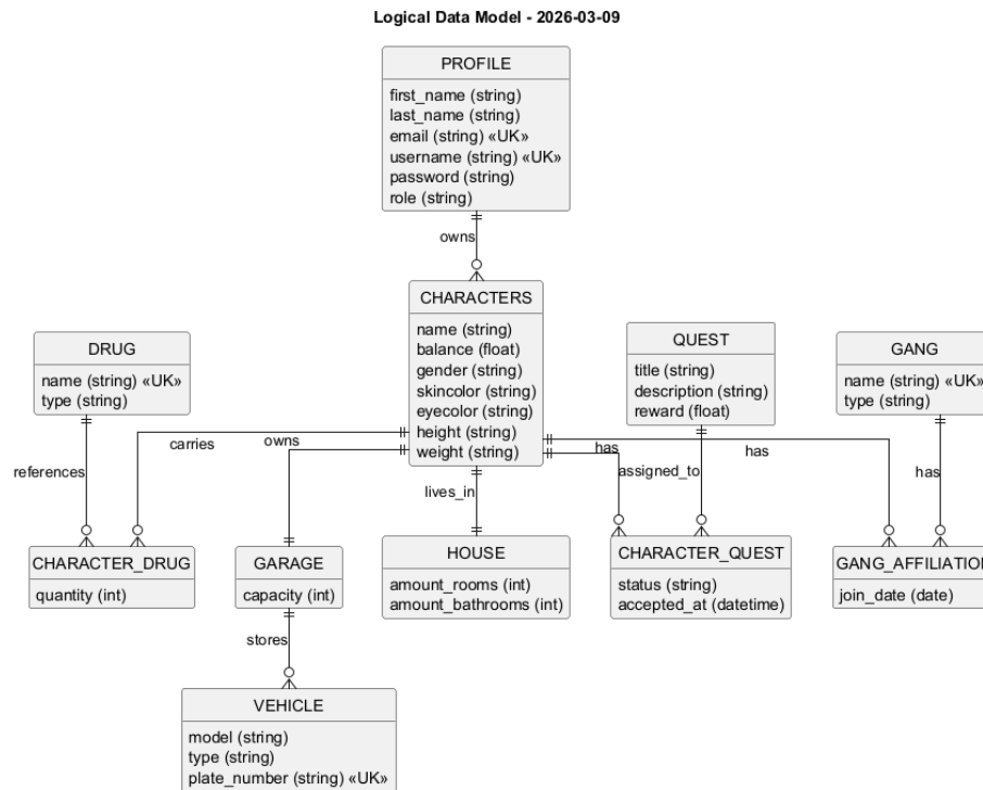
Figure 4: Logical data model. Authoritative source: 'logical-uml-09032026.puml'
