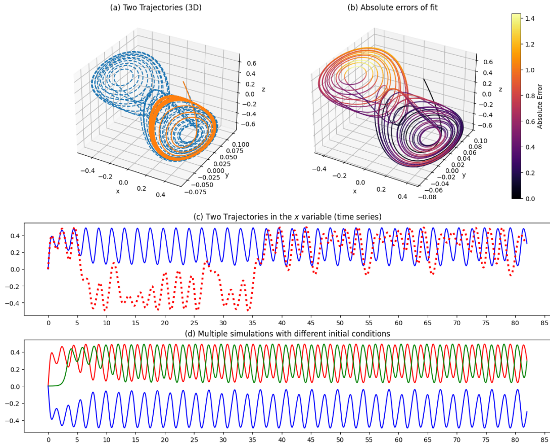
Figure 5.2.17: Experiment 3: Baseline SINDy only for \dot{x} , as in equation 5.6. For a description of this figure, refer to caption of figure 5.2.16
