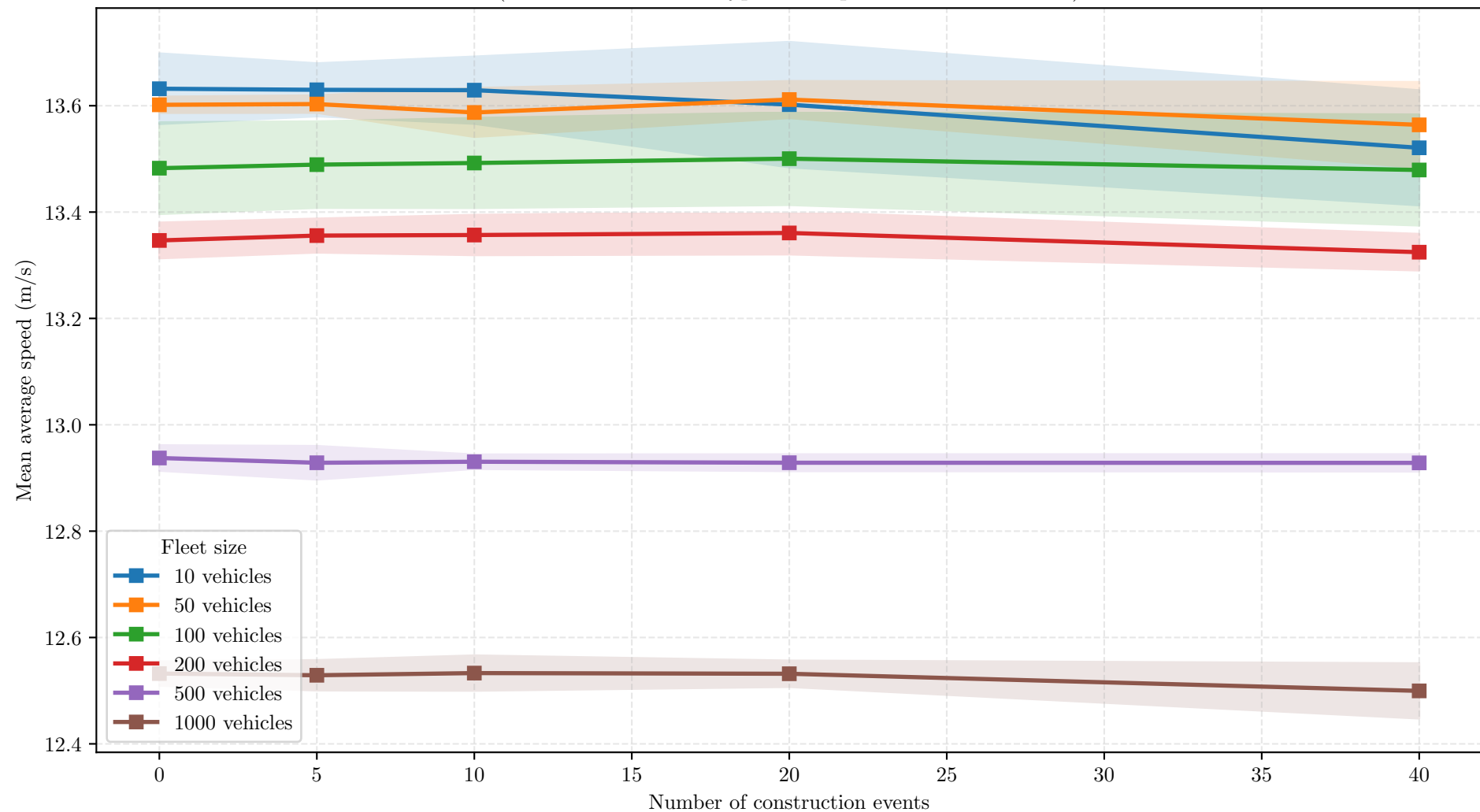
Average speed vs construction events (mixed construction types with probabilistic selection)
