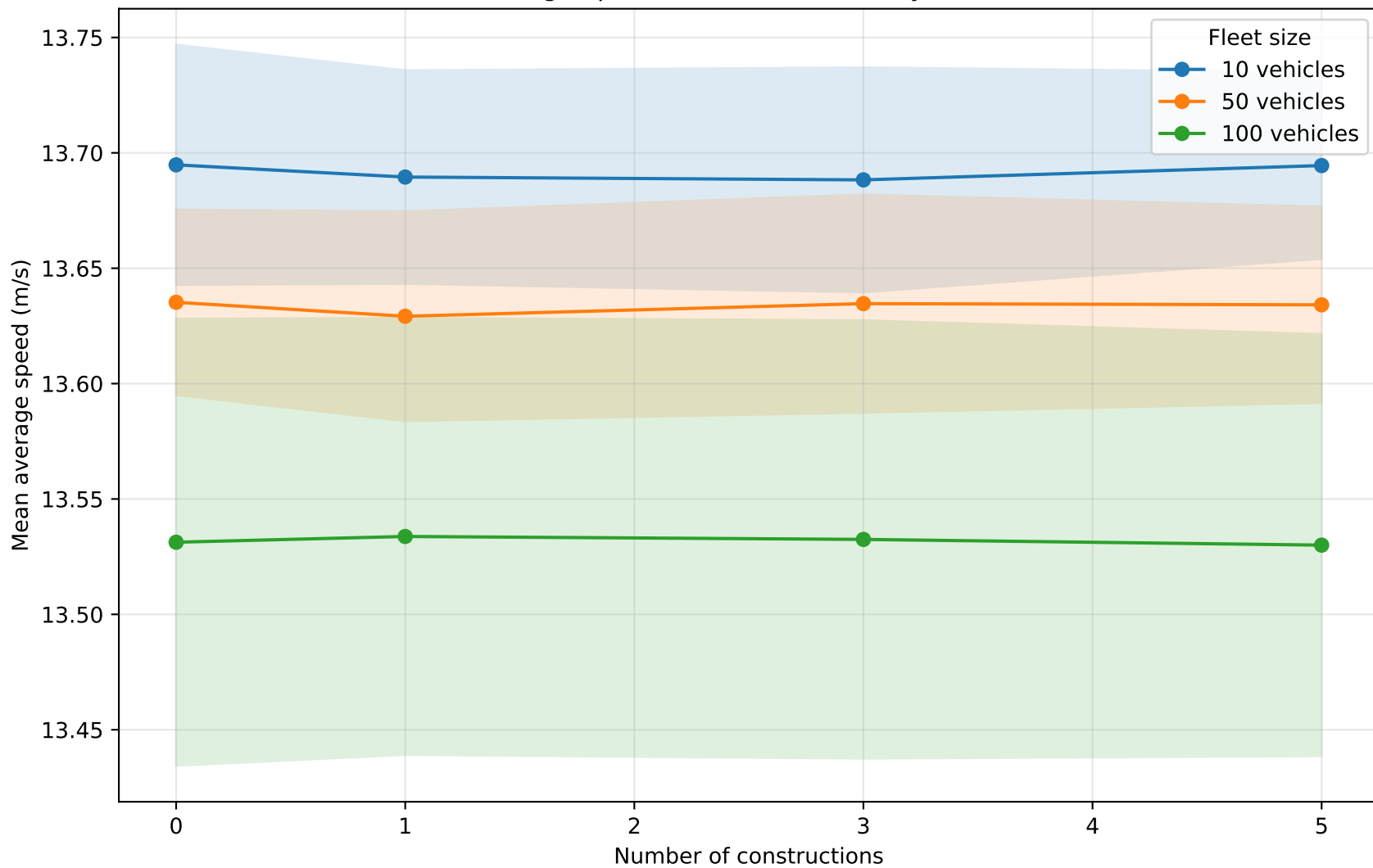
Mean average speed vs constructions by vehicle count
