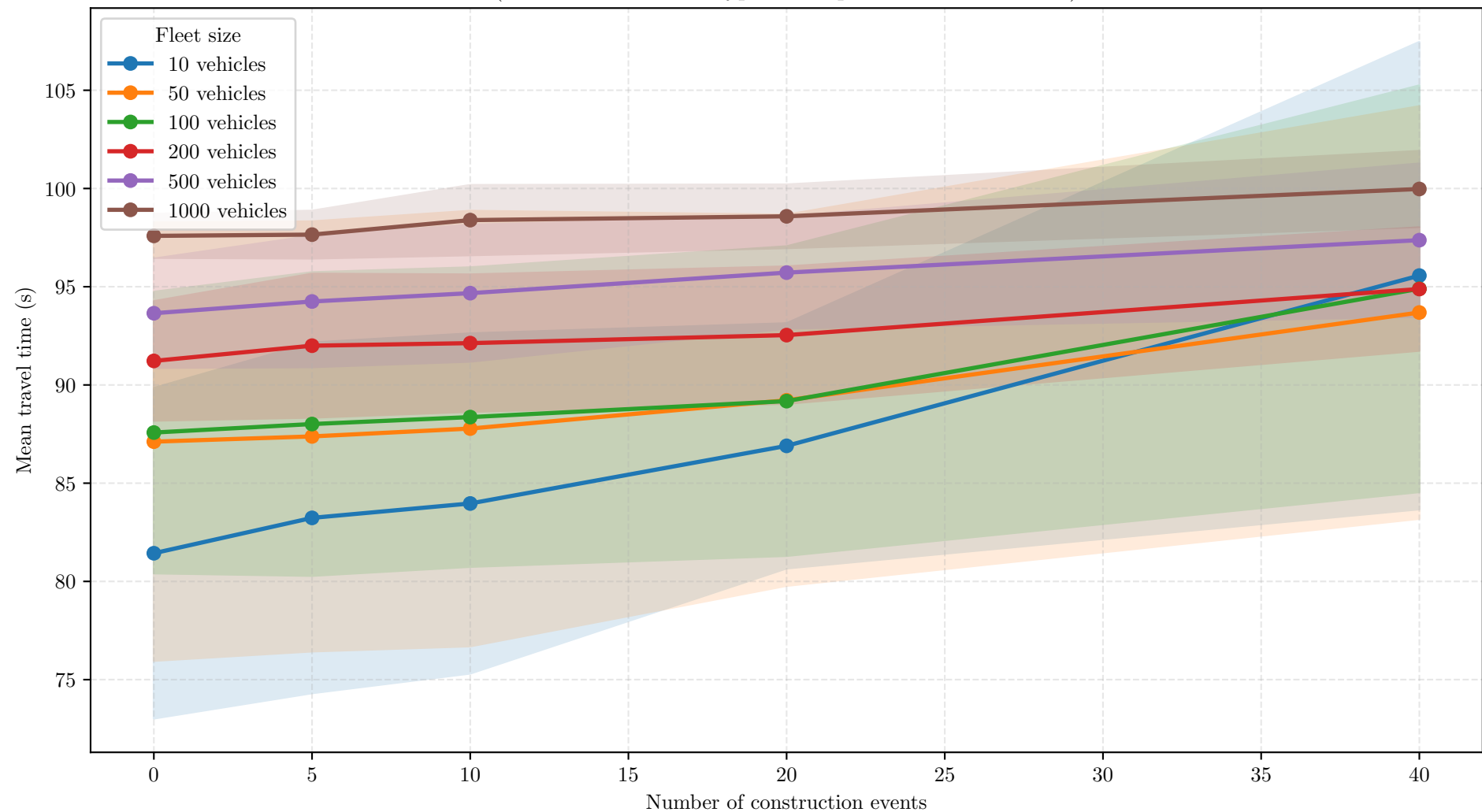
Travel time vs construction events (mixed construction types with probabilistic selection)
