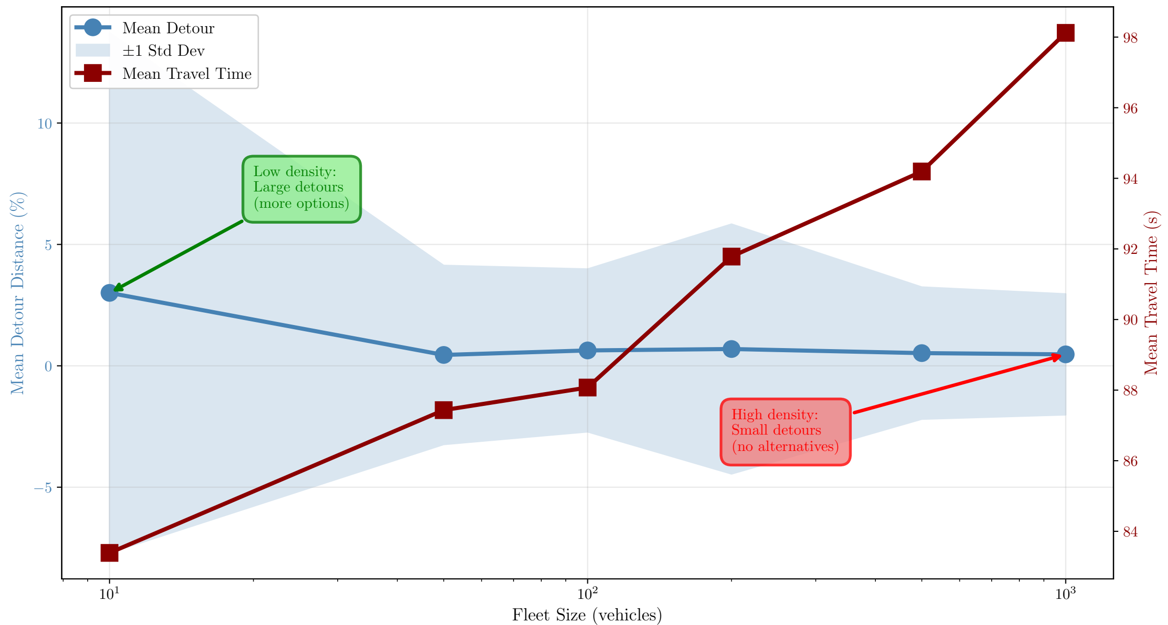
Mean Detour Distance and Travel Time vs Fleet Size
