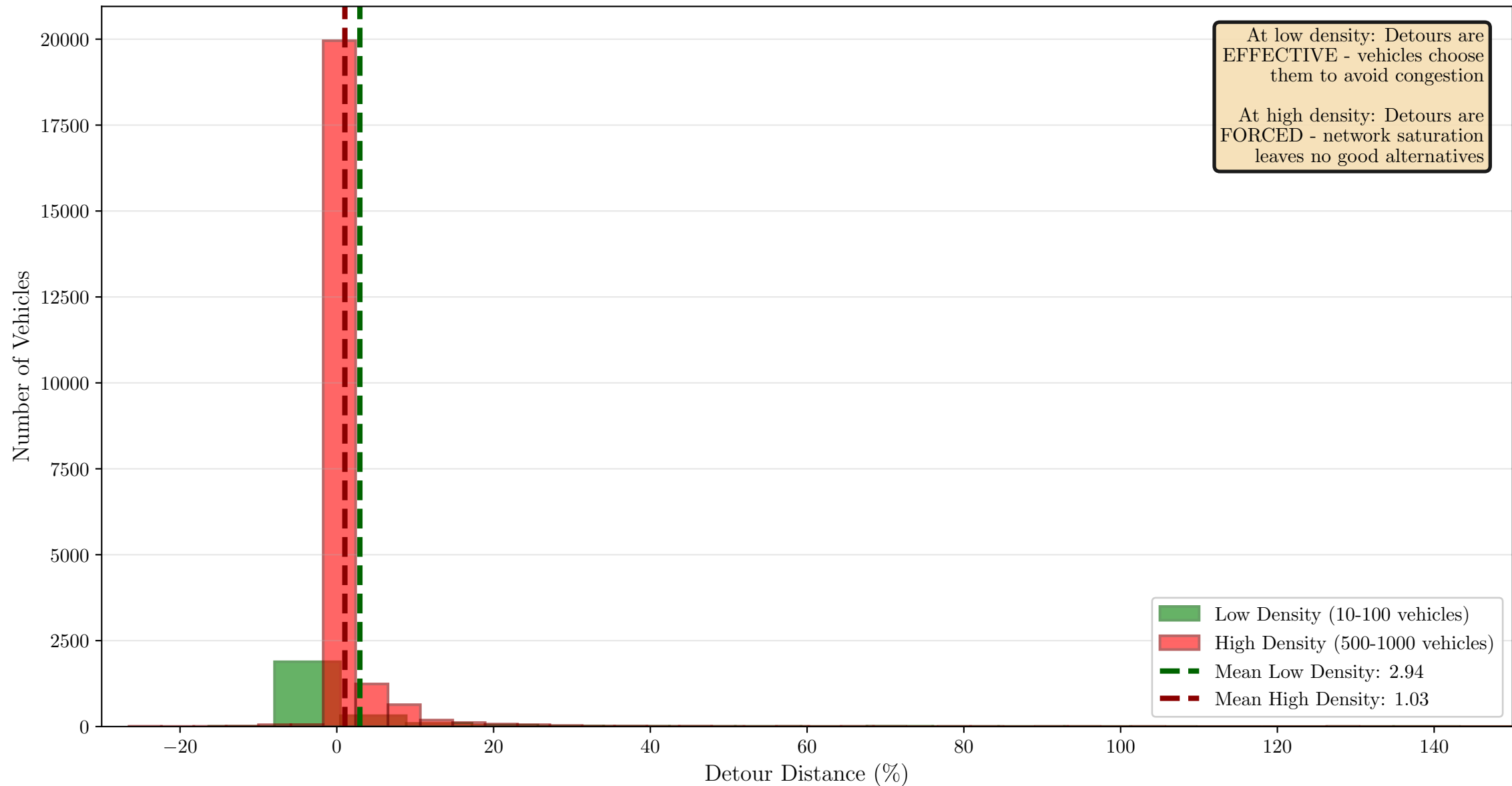
Detour Distance vs Vehicle Count Distribution Low Density vs High Density
