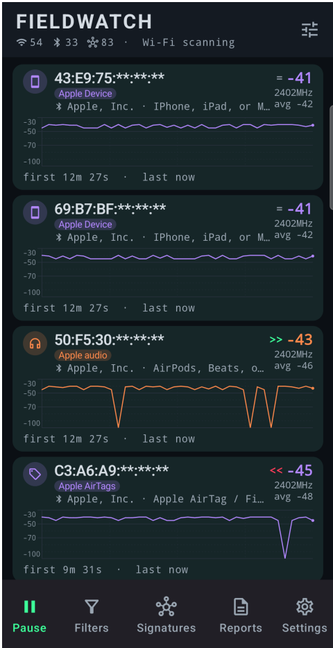
Fig. 1 — Live display (hybrid). Header is FIELDWATCH plus Wi-Fi / Bluetooth / signatures icons with counts. Circle is the signature class (unmatched = ?). Title is the MAC; Privacy mode hides the last three octets. A Wi-Fi or Bluetooth icon on the subtitle is radio kind (access point vs BLE advertiser). The number is RSSI (loudness here, not meters). Sparkline is RSSI over packets; RSSI bars off. Tune (top right) is Display. Bottom Pause freezes the picture. Privacy mode is on: last three MAC octets show as **:***.
