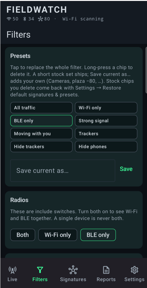
Fig. 14 — Filters, top. Presets section (eight stock chips, two across) then Radios. A tap replaces the whole filter. Save current as... is under the chips. BLE only is selected here. Privacy mode is on: last three MAC octets show as **:**:**.
