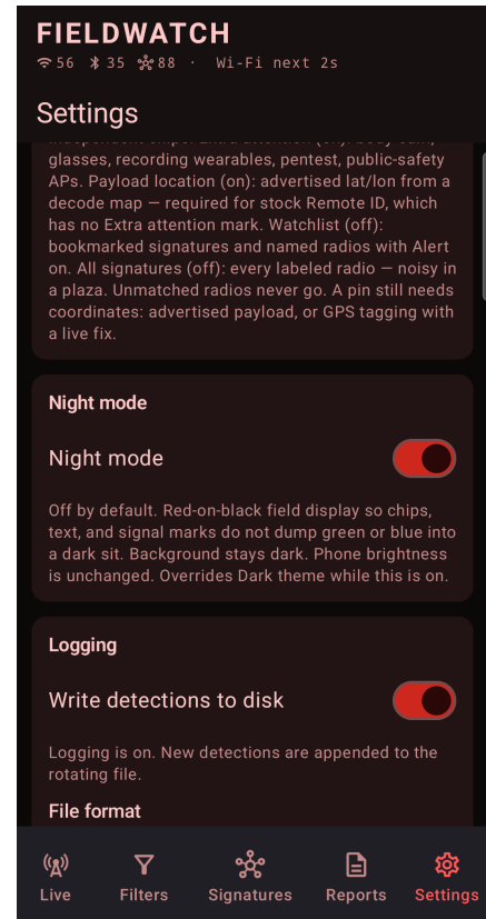
Fig. 8 — Settings → Night mode (on). Red-on-black field display. The card sits under TAK / CoT, above Logging. Phosphor switches and chips become red. Phone brightness is unchanged. Fig. 7 is the same Settings tab with Night mode off. Privacy mode is on: last three MAC octets show as ***.***
