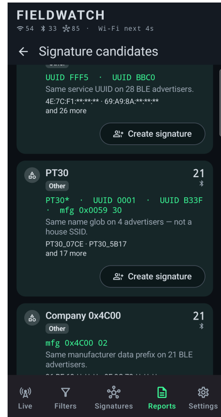
Fig. 6 — Signature candidates. Ranked families from the rotating log. Skipped randomized / house-like names. Create signature opens a draft (shared rule, no MAC pin). Privacy mode masks MAC tails. Privacy mode is on: last three MAC octets show as **:**:** .
