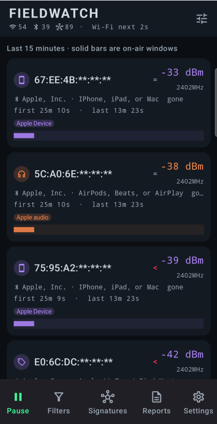
Fig. 11 — Live display, Timeline. 15-minute presence bar under each radio. Solid = on-air. MAC tails hidden (Privacy mode). Privacy mode is on: last three MAC octets show as ***:***.
