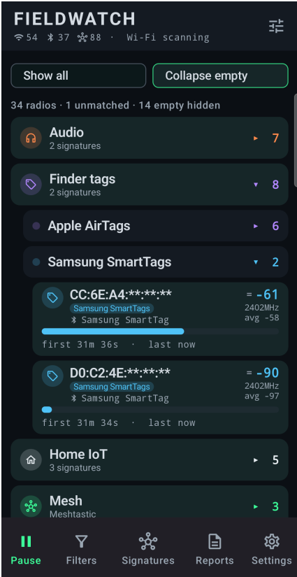
Fig. 13 — Live display, By class. Class glyph on each header (unmatched = ?). Show all keeps empty classes; Collapse empty hides zeros. Open a class, then a signature, then a radio. Radio rows use the same class glyph and Display switches as the list. Privacy mode is on: last three MAC octets show as ***:**.
