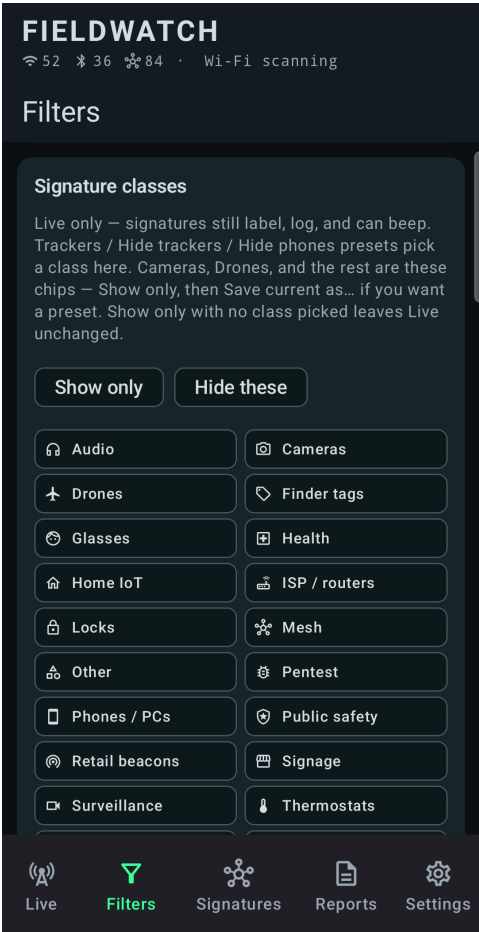
Fig. 15 — Filters, Signature classes. Show only / Hide these plus two-across class chips (Health, Public safety, ...). Show only selected / Hide selected open a list of families further down. Privacy mode is on: last three MAC octets show as **:**:**.
