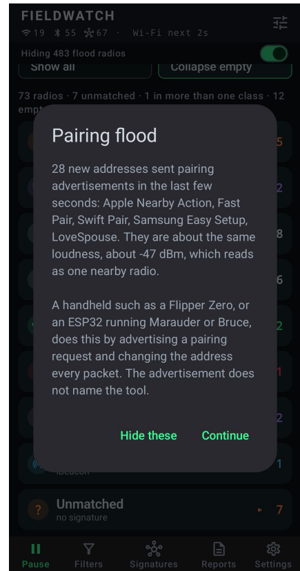
Fig. 1 — Pairing flood. Hide these takes those new addresses off the Live display. Continue leaves them up. The line behind the dialog is an earlier burst still hidden.
