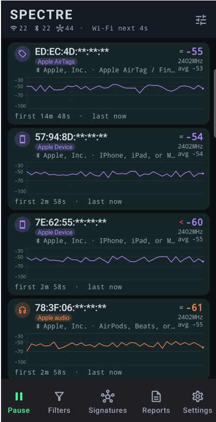
Fig. 10 — the Live display, Hybrid. Strength list plus RSSI sparkline (fixed −30 to −100 dBm). RSSI bars off so the sparkline is the strength picture. Fig. 1 is this view too. Privacy mode is on: last three MAC octets show as ***:***:***.
