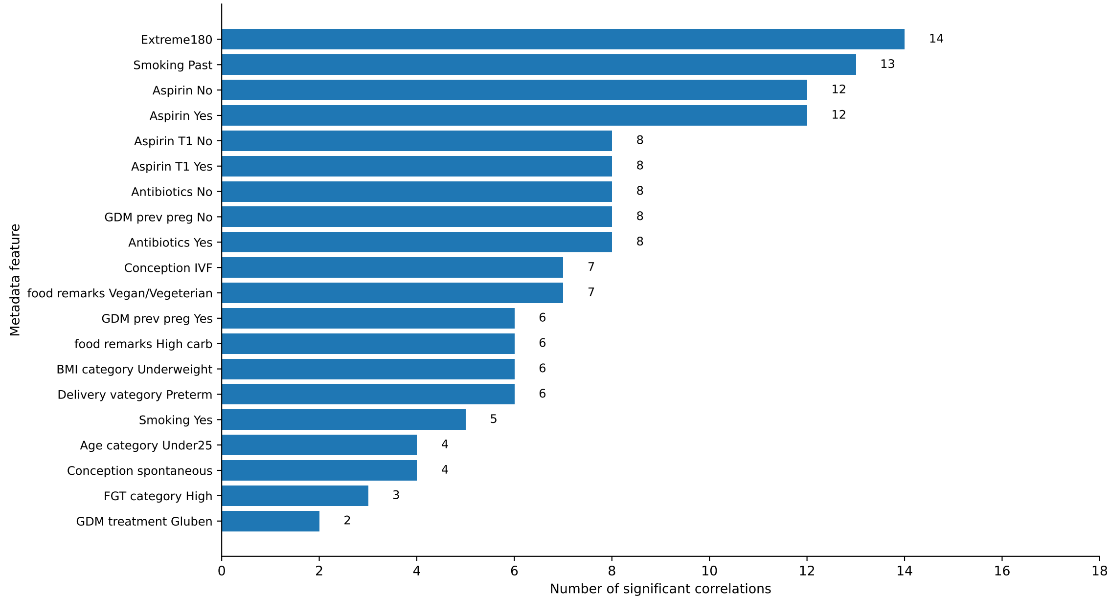
omri_stool_Pregnant_16S Significant microbe-metadata correlations, FDR-adjusted p < 0.05
