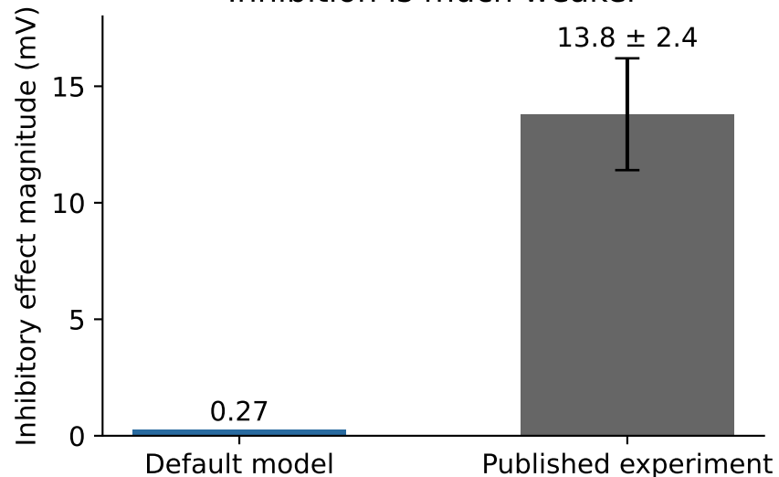
Inhibition is much weaker
