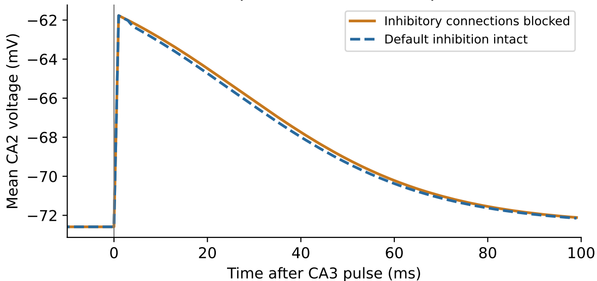
Responses almost overlap
