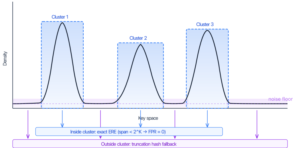
Figure 5.1: Segmented ARE filter: dense clusters go into exact-mode sub-filters ( \text{FPR} = 0 ); sparse keys between clusters go to a fallback.
