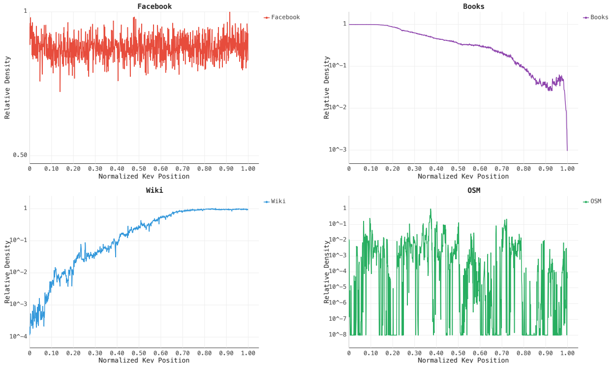
Figure 3.1: Key density histograms for SOSD datasets (1000 bins, log-scale Y-axis). Each bin’s value is the fraction of keys falling in it, divided by 1/1000 , so the uniform distribution gives 1 everywhere.
